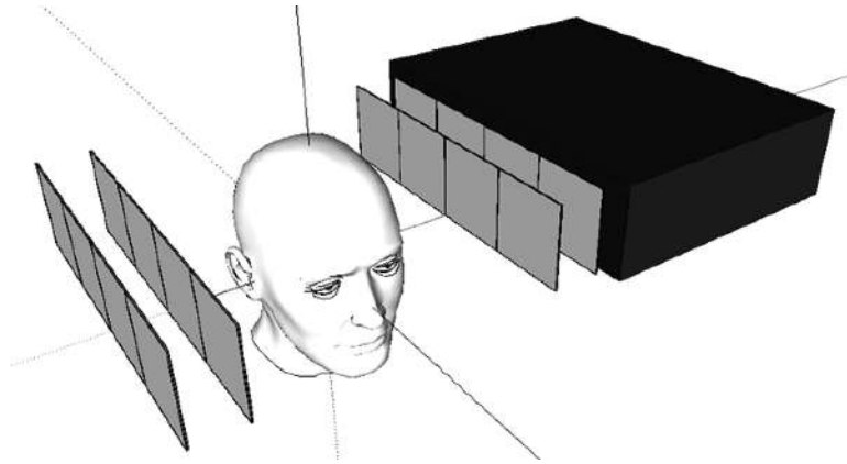
Fig. 1. Layout of the pCT head scanner under construction. A proton entering from the left is first tracked in the entrance telescope of two x-y planes of silicon strip sensors, and after passing through the phantom/patient, in the similarly constructed exit telescope, before its residual energy/range is determined in the energy detector.
