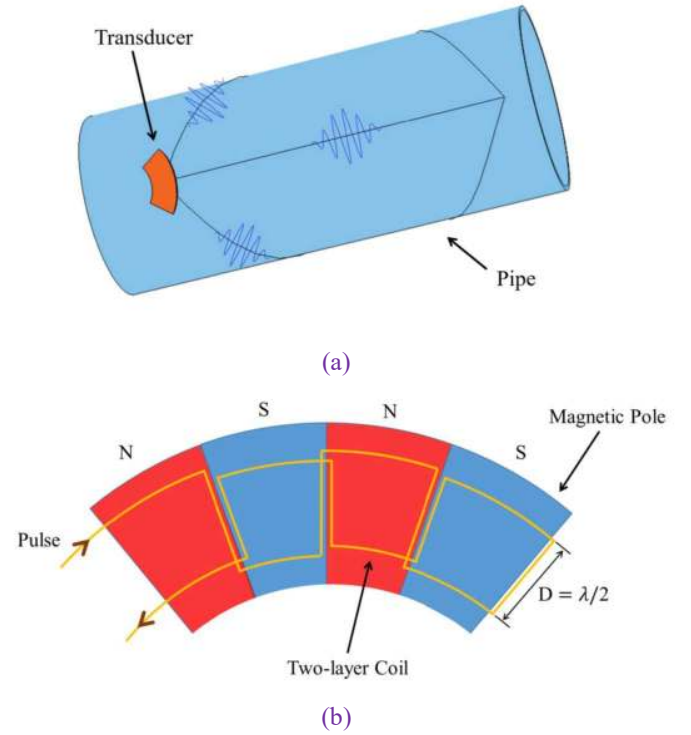
Fig. 1 The designed transducer for helical Lamb wave. (a) The wave propagating in direct and spiral way. (b) The detailed depiction of the transducer structure.
