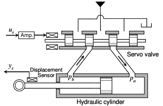
Fig. 6: Schematic diagram of hydraulic cylinder
