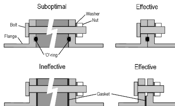
Figure 6. Typical flange connections for thermoacoustic pipe systems.
