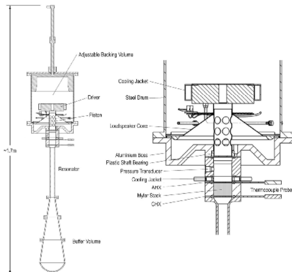
Figure 1. General layout of the loudspeaker-driven thermoacoustic refrigerator (TAR).
