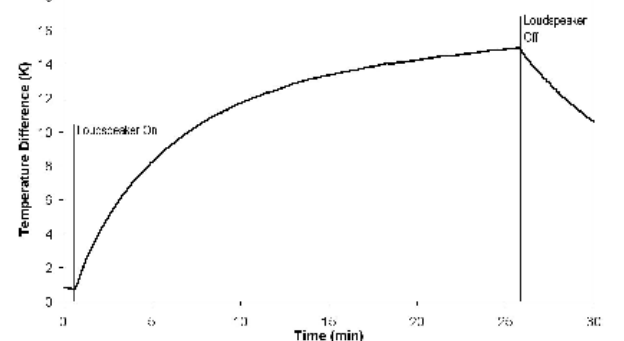
Figure 8. Measured TAR AHX/CHX temperature difference over time using 700kPa air.
