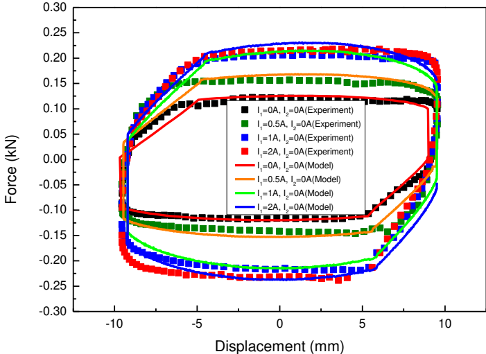
Fig.16. Identification results of variable damping
