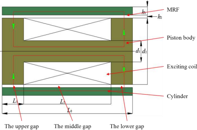
Fig. 2. The sketch of the damping unit
