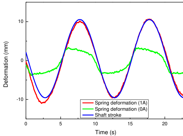
Fig. 9. Spring deformation under different currents.
