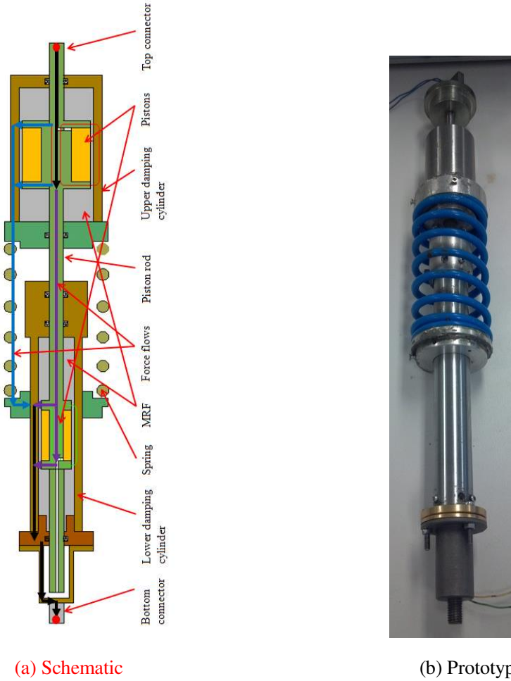
Fig.1. Design drawing and prototype of the MRF damper: (a) schematic; and (b) prototype.
