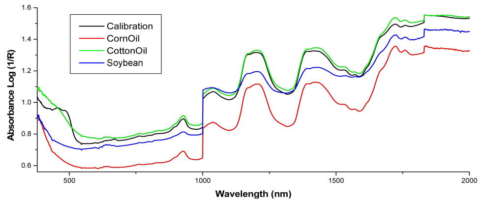
Figure 1. An overlaid spectral virgin sunflower oil (calibrator) with different oils (corn, cotton, and soy oil) showing absorbance (log 1/R) against wavelength in nanometers after pretreatment.
