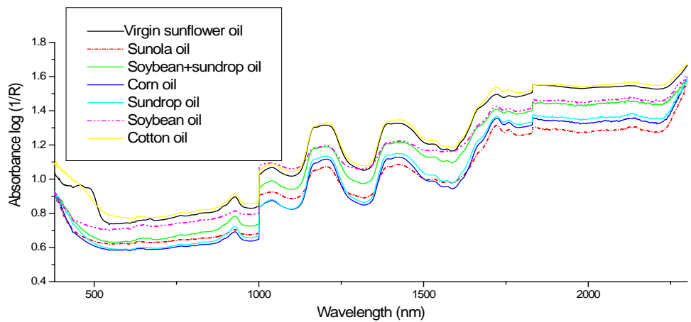
Figure 3. An overlaid spectral virgin sunflower oil (calibrator) with different oils (sunola, sundrop, corn, cotton, and soy oil) showing absorbance (log 1/R) against wavelength in nanometers after pretreatment.
