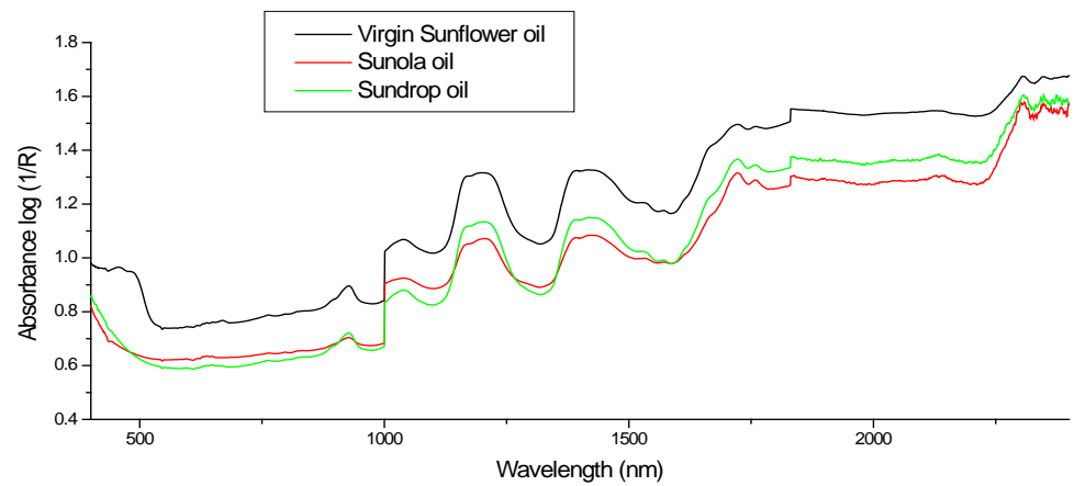
Figure 2. An overlaid spectral virgin sunflower oil (calibrator) with different oils (sunola and sundrop oil) showing absorbance (log 1/R) against wavelength in nanometers after pretreatment.
