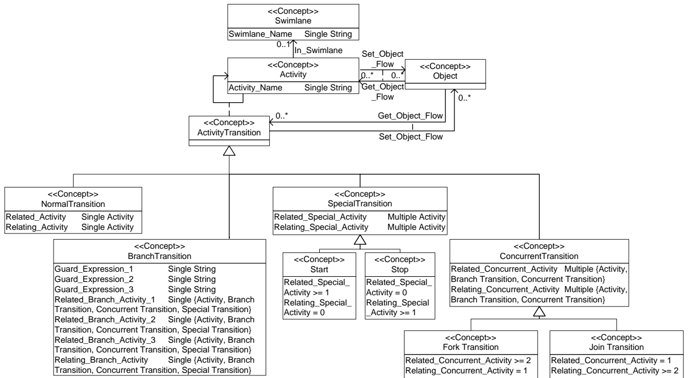
Fig. 10. UML activity diagram ontology
