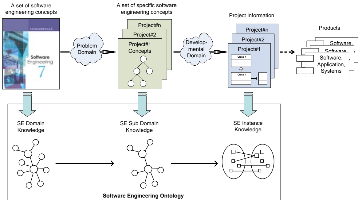
Fig. 1. Schematic overview of software engineering knowledge representation
