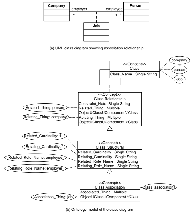
Fig. 7. Presentation of instances of classes and properties
