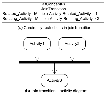
Fig. 5. Class JoinTransition presentation and its properties
