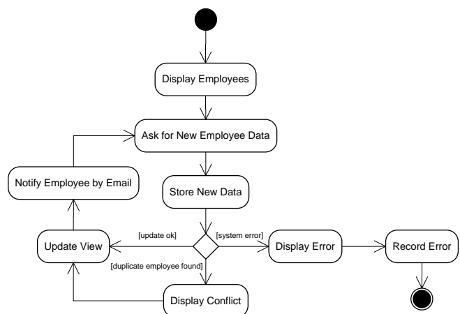
(a) A revised design of activity diagram
