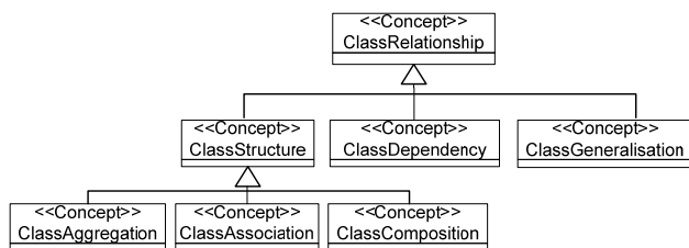
Fig. 2. Class ClassRelationship presentation and its sub-classes
