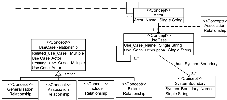
Fig. 11. UML usecase diagram ontology
