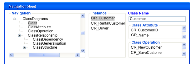
(a) Class instance CR_Customer
