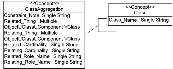
Fig. 6. Association class ClassAggregation presentation
