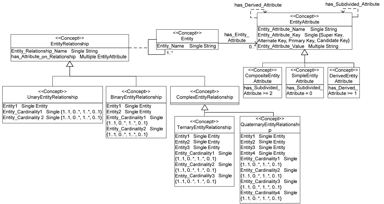
Fig. 9. Entity diagram ontology
