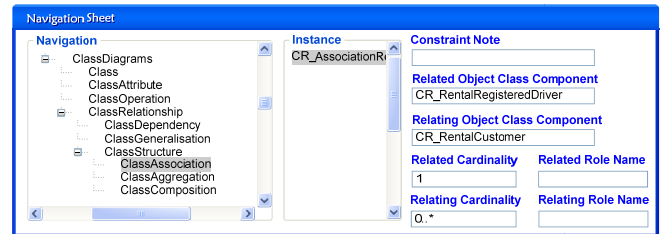
(b) ClassAssociation instance CR_AssociationRelationship
