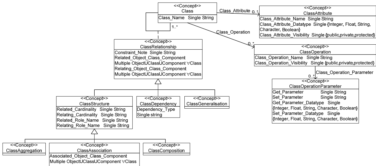
Fig. 8. UML class diagram ontology
