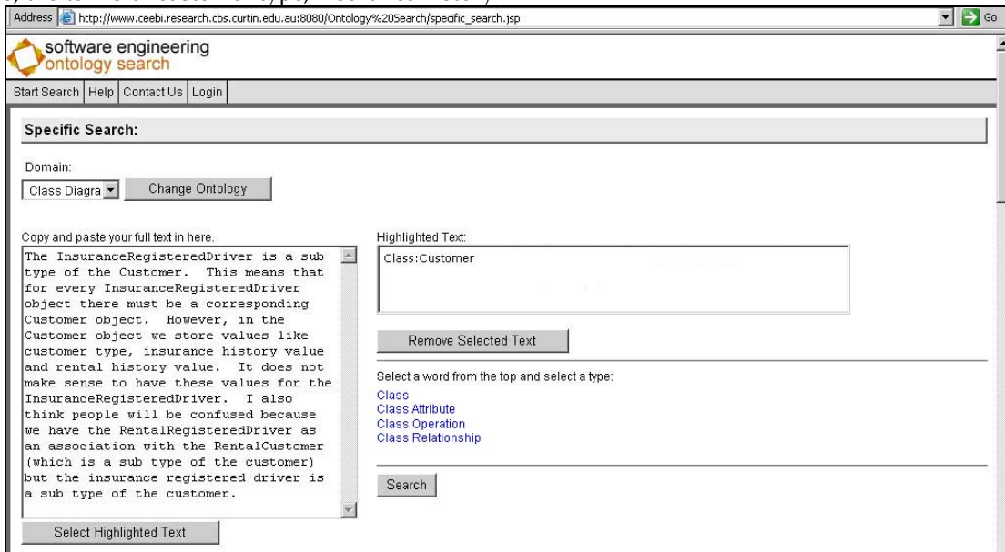
Fig. 16 An example of annotating 'customer' as class
