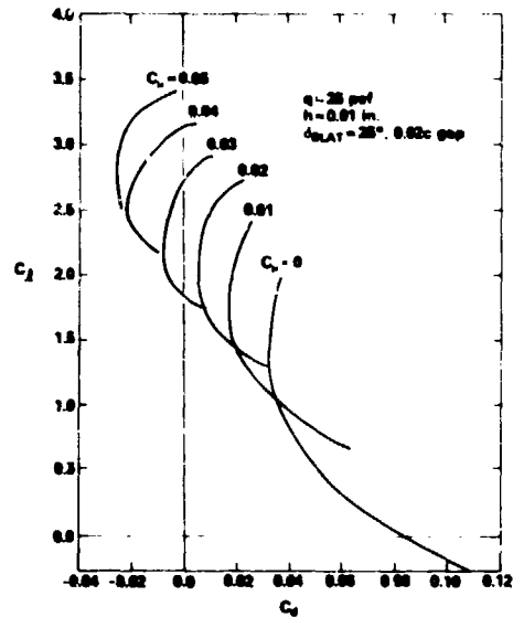
Fig. 22 - Drag Polars at Constant Blowing for Dual Radius CCW Configuration A, c_f = 0.0223c'
