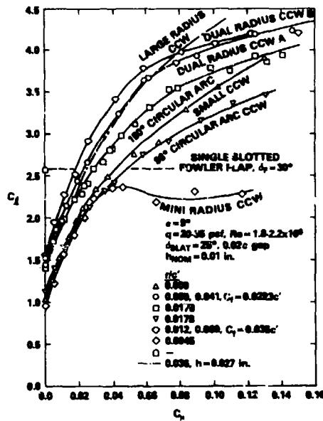
Fig. 18 - Comparative Blown Lift Configurations
