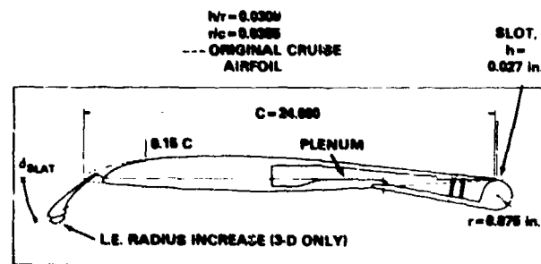
Fig. 1 - A-6/CCW Wing-Fold Airfoil Section (64A008.4/CCW), \delta_{SLAT} = 37.5^\circ , Large Trailing Edge Radius
