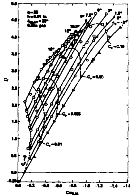
Fig. 23 - Pitching Moment of the Dual Radius CCW Configuration B, c_f = 0.0335c'
