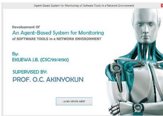
Figure 5: Welcome Screen
