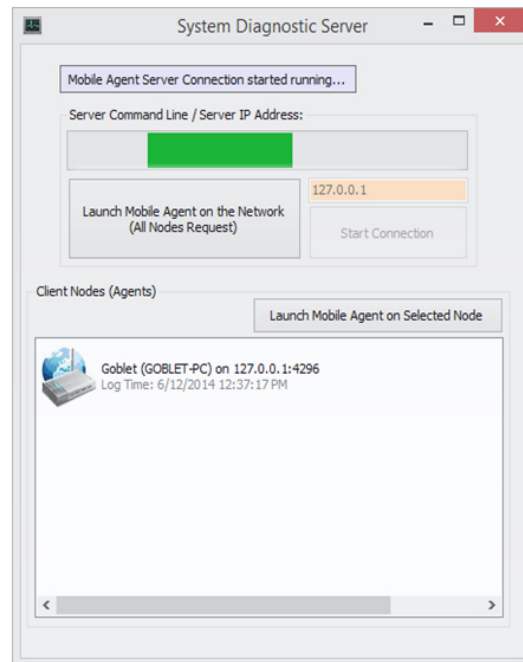
Figure 6: Welcome Screen
