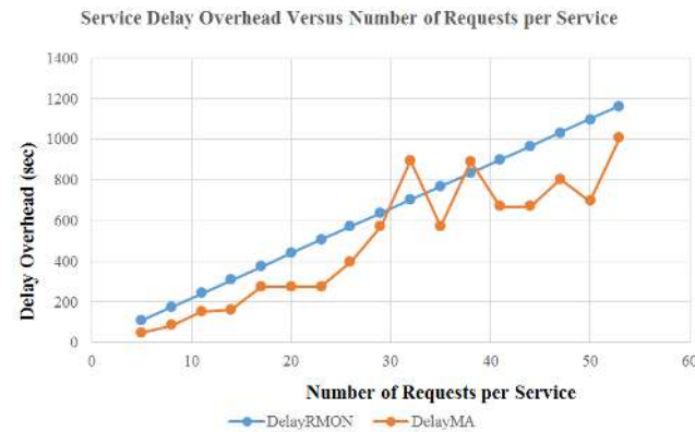
Figure 16: Service Delay Versus Number of Requests per Service
