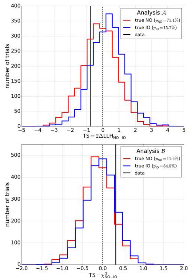
Fig. 10 Distribution of the TS from PTs, generated with the best-fit systematic parameters \eta^{NO} and \eta^{IO} from Table 2 for Analysis A (top) and Analysis B (bottom). The red and blue distributions are obtained for the NO and IO hypotheses, respectively, while the black, solid vertical line shows the observed value in data, giving the p -values for the NO and IO hypotheses stated in the legends
