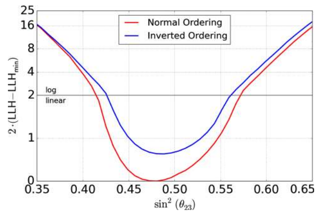
Fig. 11 The negative log-likelihood (LLH) as a function of \sin^2(\theta_{23}) for Analysis A, relative to the global minimum LLH_{min} . The preference for NO over IO is visible over all the range of \sin^2(\theta_{23}) with the best-fit for both orderings being in the lower octant ( \sin^2(\theta_{23}) < 0.5 )
