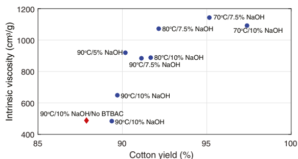
Fig. 10 Intrinsic viscosity plotted against the yield of cotton from the different PET hydrolyses in large-scale experiments. All samples in the graph were treated for 240 min except for the two samples with the lowest intrinsic viscosity, which were treated for 360 min
