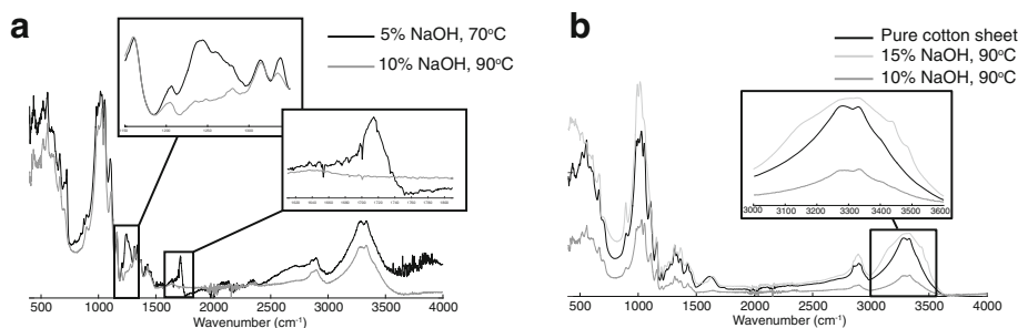
Fig. 9 ATR FT-IR spectra of the solid (cotton) residue after PET hydrolysis. In a , a comparison between a sample where only 66% of the TPA yield had been reached (5% NaOH, 70 °C, 240 min) and a sample where full yield had been reached (10% NaOH, 90 °C, 240 min) is shown. Both from large-scale experiments, 52 mmol BTBAC/kg solution. In b , a comparison between pure cotton sheets (as a reference), a sample treated in 15% NaOH (90 °C, 100 min, small-scale experiments, 52 mmol BTBAC/kg solution), and a sample treated in 10% NaOH (90 °C, 240 min, large-scale experiments, 52 mmol BTBAC/kg solution) are shown
