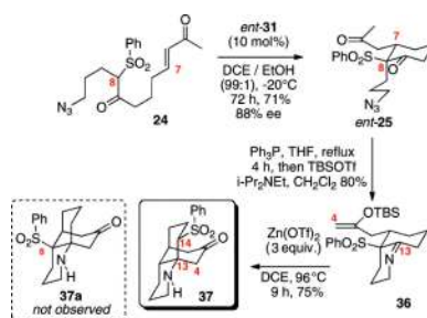
Scheme 5. Enantioselective Synthesis of the Lycopodine Tricyclic Core 37 .
