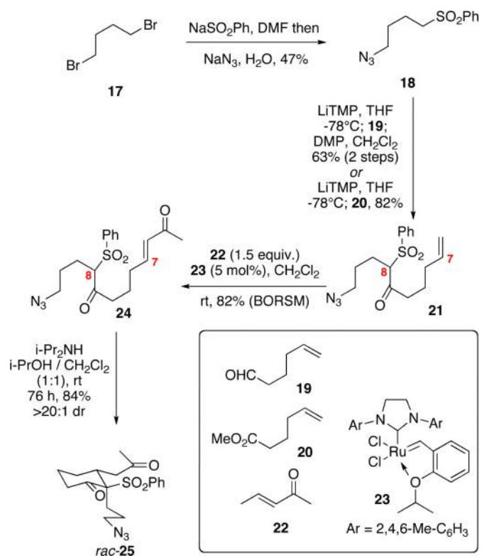
Scheme 3. Development of Racemic Protocol for Intramolecular, Keto Sulfone Michael Addition.
