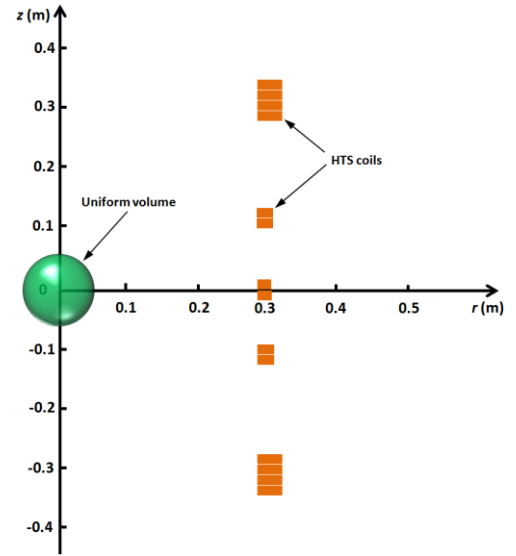
Fig. 3. The basic configuration of the HTS magnet: 5-set of double-pancake HTS coils.
