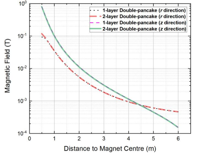
Fig. 7. Stray field (unshielded) in the r -direction and z -direction, with the ideal case of transport current 1000 A.
