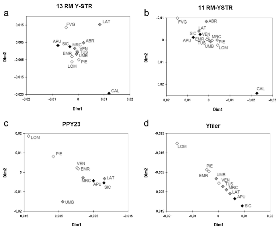
Fig. 2. Two-dimensional MDS plots of linearized F_{ST} values for: (a) 13 RM Y-STRs (Kruskal's stress = 0.150); (b) 11 RM Y-STRs (Kruskal's stress = 0.216); (c) PPY23 (Kruskal's stress = 0.200); (d) Yfiler (Kruskal's stress = 0.205). Geographical groups are identified by means of coloured diamonds: white, Northern Italy (PIE = Piedmont, LOM = Lombardy, VEN = Veneto, FVG = Friuli Venezia Giulia, EMR = Emilia Romagna); grey, Central Italy (TUS = Tuscany, UMB = Umbria, MRC = Marche, LAT = Latium, ABR = Abruzzo); black, Southern Italy (APU = Apulia, CAL = Calabria, SIC = Sicily).
