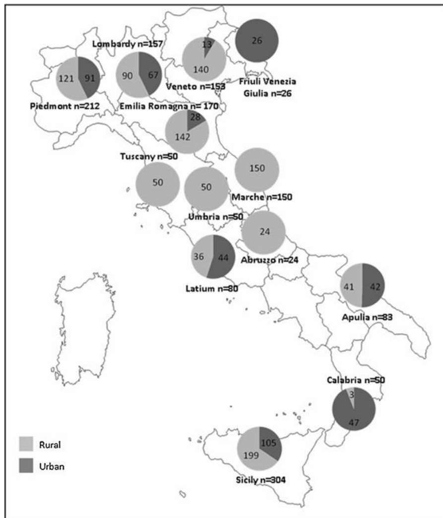
Fig. 1. Geographic localization and characteristics (sample size, composition in terms of rural/urban origin of the tested individuals) of the thirteen Italian regional population samples analysed in the GEFI RM Y-STR study.
