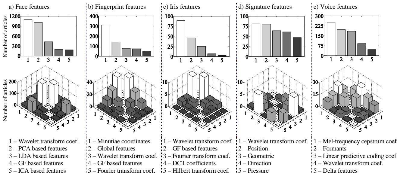
Fig. 2. Number of articles naming five most frequently used biometric features and their mixtures (PCA – principal component analysis, LDA – linear discriminant analysis, GF – Gabor filters, ICA – independent component analysis, DCT – discrete cosine transform)
