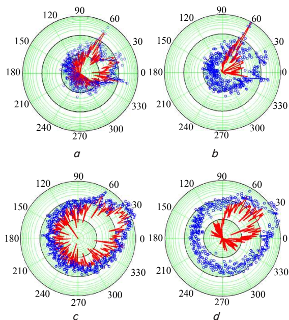
Fig. 5. Current angular spectra of communication characteristics of multipoint one-beam ( a, b ) and eight-beam ( c, d ) WE depending on the direction of reception at fixed value of initial angle -30^\circ of radiation beam for the case of transmitting and receiving aerial arrays: a, c – isotropic aerial elements; b, d – directional aerial elements
