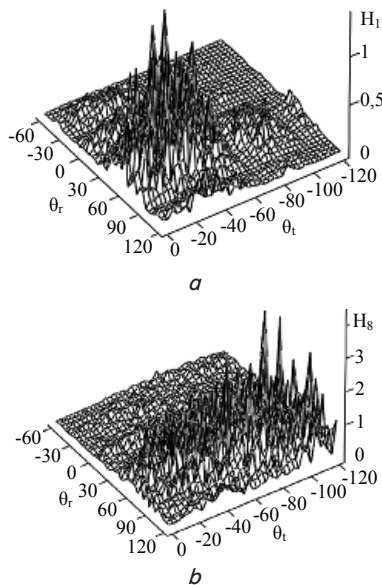
Fig. 1. Communication characteristics of tested two-point WE: a – in the case of one beam of radiation and reception; b – in the case of eight different beams of radiation and reception
