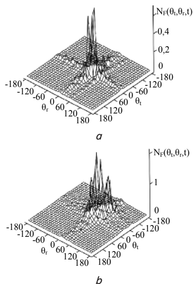
Fig. 3. Communication characteristics of multipoint wireless environment: a – in the case of one radiation beam and one reception beam; b – in the case of eight different beams of radiation and reception
