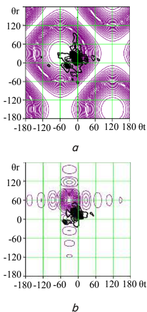
Fig. 4. Comparison of communication characteristics of different types of multipoint one-beam wireless environments: a – direct determined beams; b – indirect determined beams
