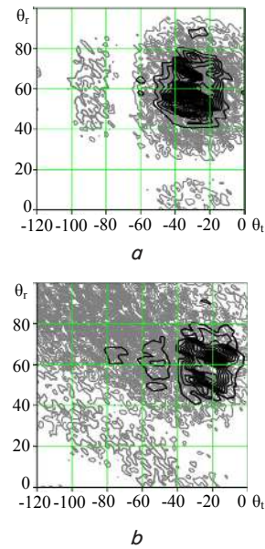
Fig. 2. Communication characteristics of two-point WE without (gray color) and with taking into account the use of directional aerials at the transmitting and receiving sides (black color): a – in the case of one radiation beam and one reception beam; b – in the case of eight different beams of radiation and reception
