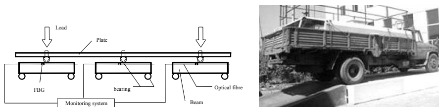
Figure 7 Weight in motion based on FBG
