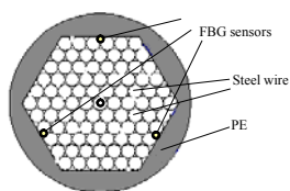
Figure 6 Smart cables based on FBGs
