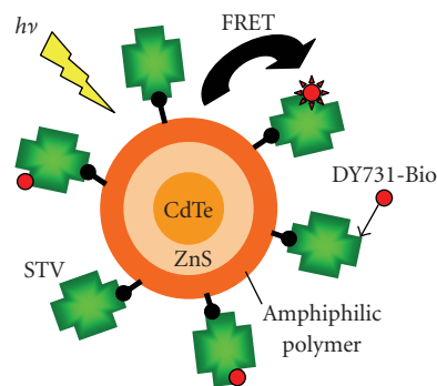
FIGURE 1: Schematic diagram of Qdot705-STV and DY731-Bio in self-assembled assay where energy can be transferred nonradiatively from QD to DY731-Bio upon excitation.
