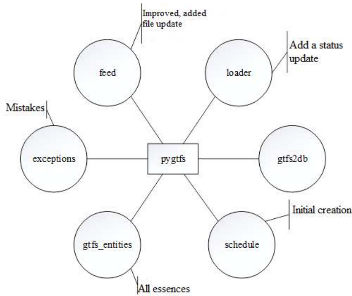
Figure 29: The structure of the pygtfs module with its modification
