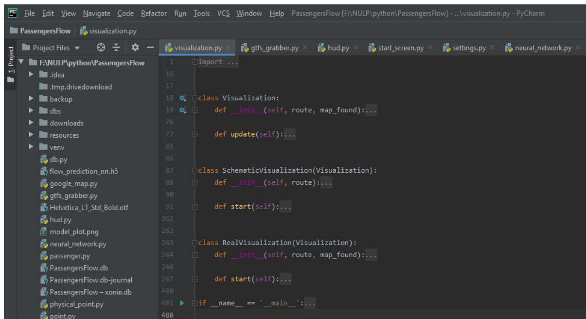
Figure 39: PyCharm window
