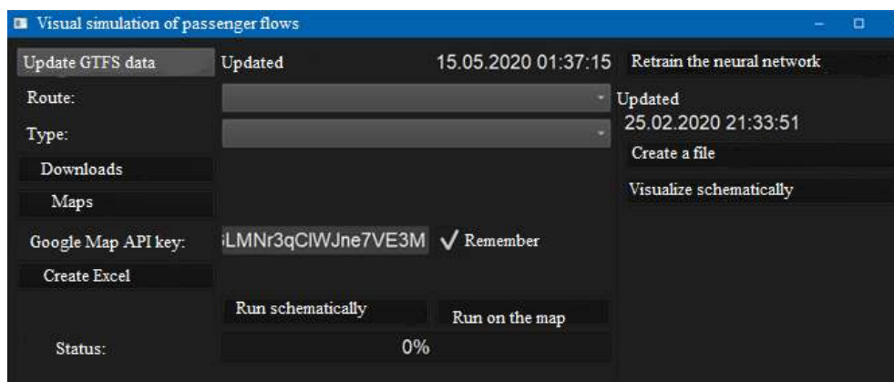
Figure 62: Main interface
