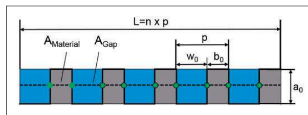
Figure 4. Surface of identical rectangle model.
