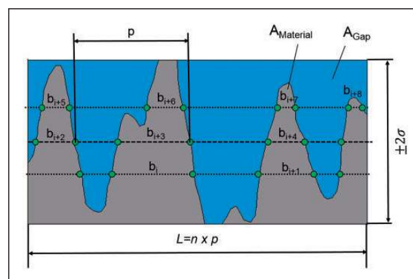
Figure 5. Surface of identical rectangle model.
