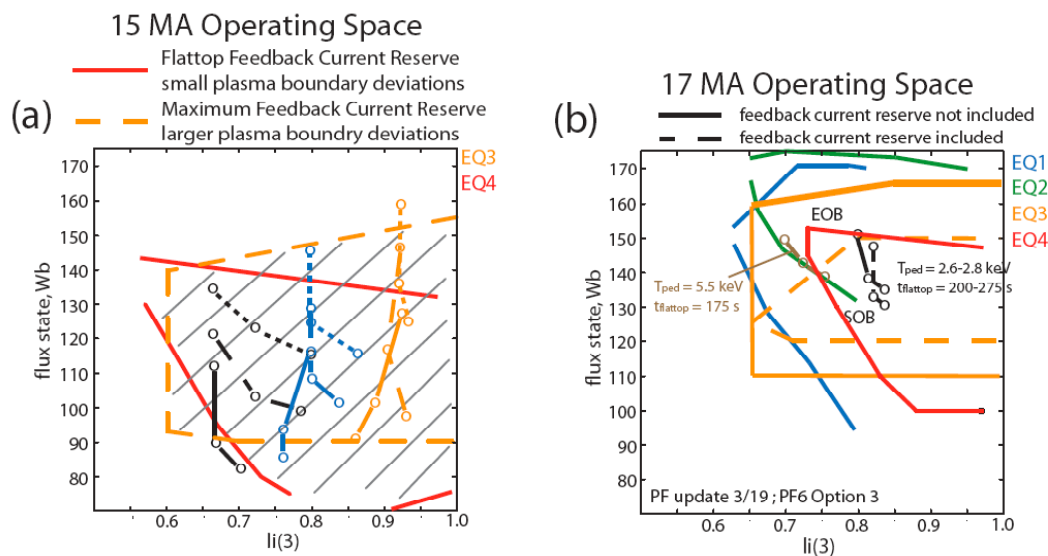
Figure 3. Flux state versus I_i operating space diagrams including flattop and maximum feedback current reserve (a), and 17 MA scenario (b).
