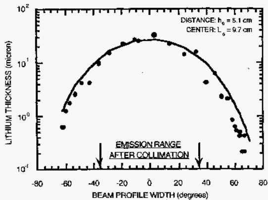
Fig. 5 The results of off-line measurements in a vacuum chamber obtained with and without the collimation required to restrict the lithium deposition to Inner Limiter. The solid line is the result of a least-squares-fit of first order evaporation theory to the measured angular distribution.
