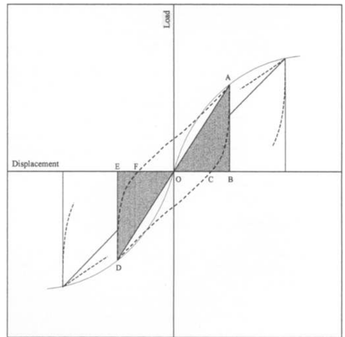
Fig. 7. Method of obtaining equivalent viscous damping
