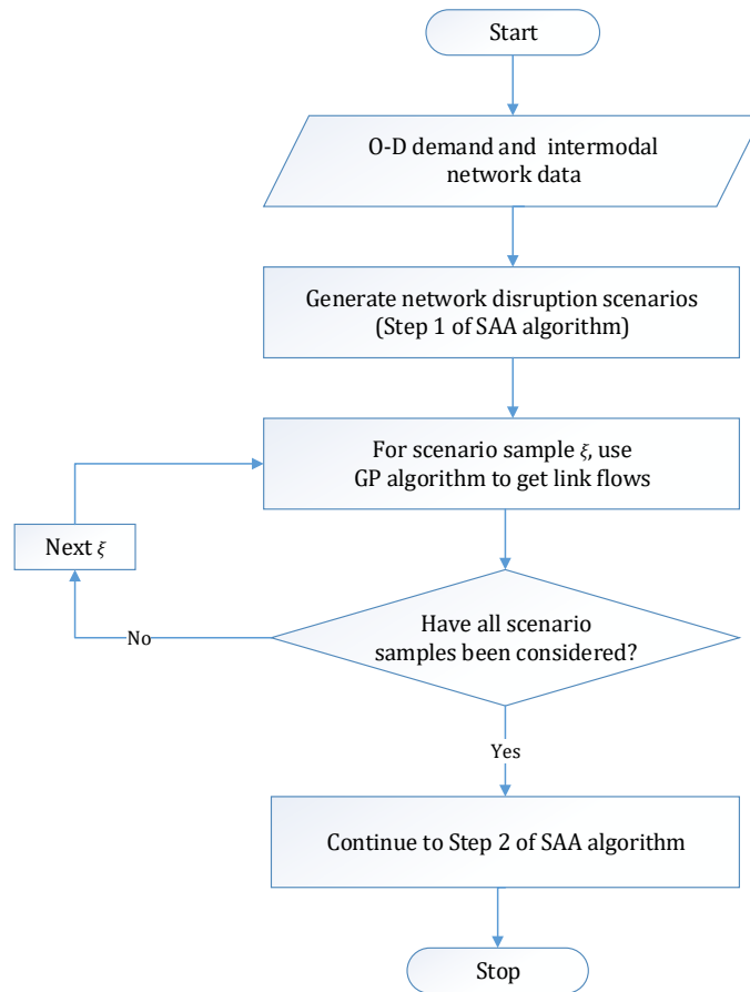
Figure 3.1 Algorithmic framework.
