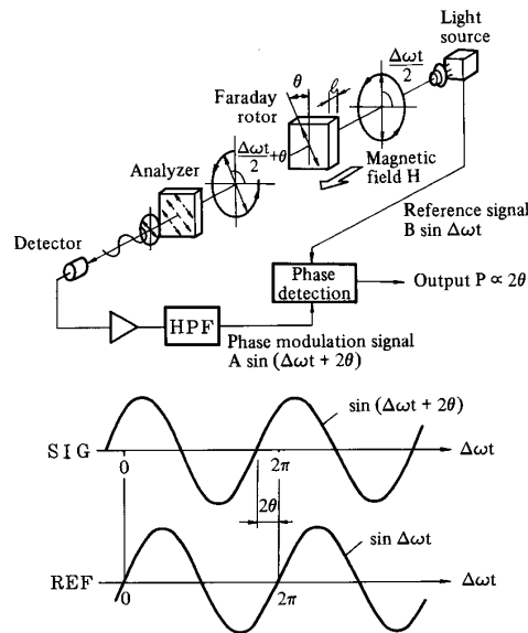
Fig. 3 Principles of light power phase detection system
