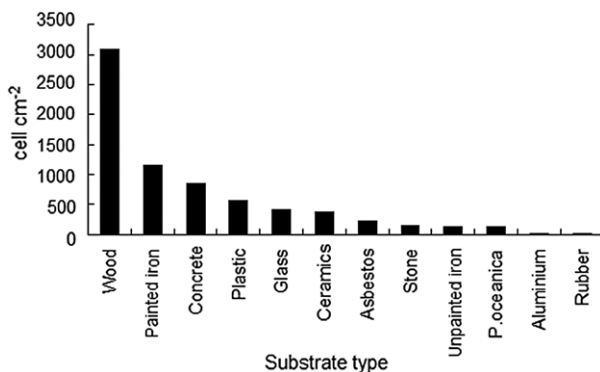
Fig. 3. Cylindrotheca closterium abundance on top sides of examined substrates.
