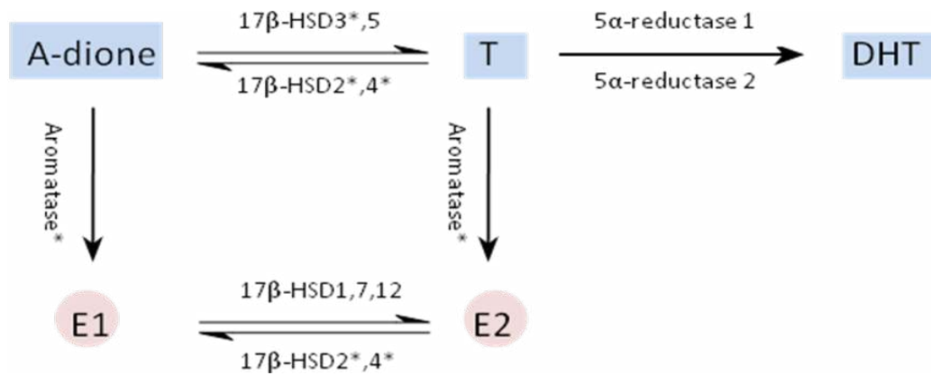
Figure 6: Extragonadal pathways of androgens (boxes) and estrogens (circles). Asteriks indicate the enzymes that are present in osteoblasts
