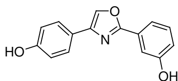
IC_{50} (HSD2) = 249 nM
