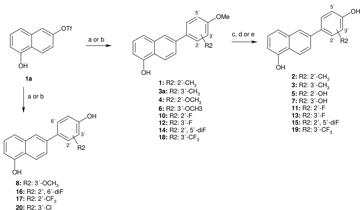
Scheme 1. Synthesis of compounds 1 to 8 and 10 to 20 a
