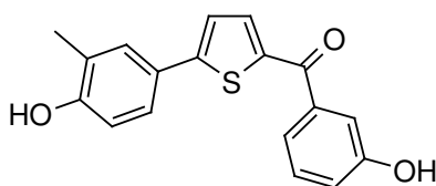
Figure 12: Starting point of a new class of 17β-HSD2 inhibitor (Chapter 3.III)
