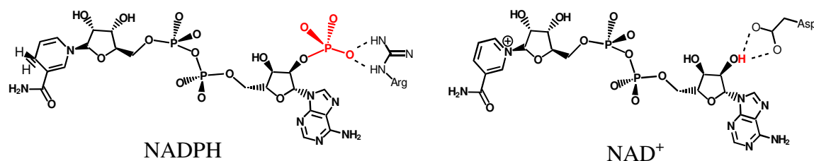
Figure 4: Cofactor preference for reductive (NADPH) and oxidative (NAD + ) 17\beta -HSDs
