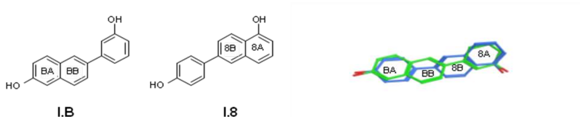
Figure 14: Superimposition of compounds I.B and I.8
