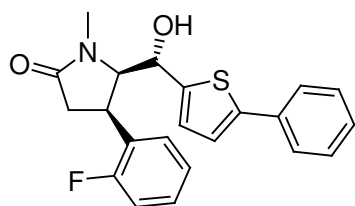
Pyrrolidinone IC_{50} (HSD2) = 10 nM
