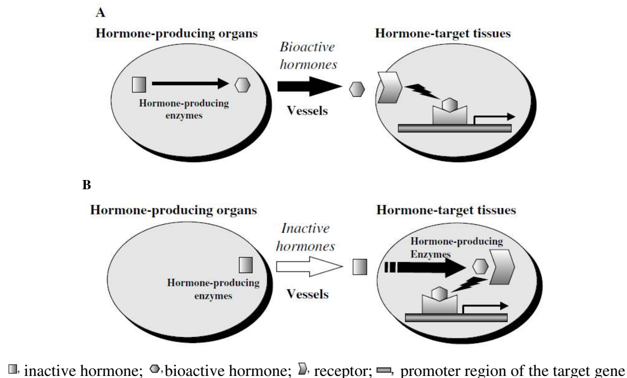
Figure 1: Representation of endocrine (A) and intracrine (B) concept (taken from Suzuki T. et al. 9 )
