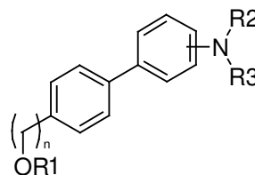
Figure 11: Structure overview of the molecules reported in this thesis
