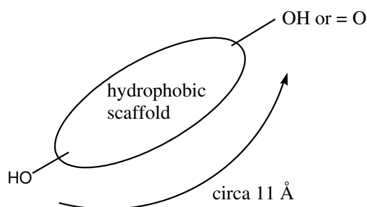
Figure 10: Simple pharmacophore model
