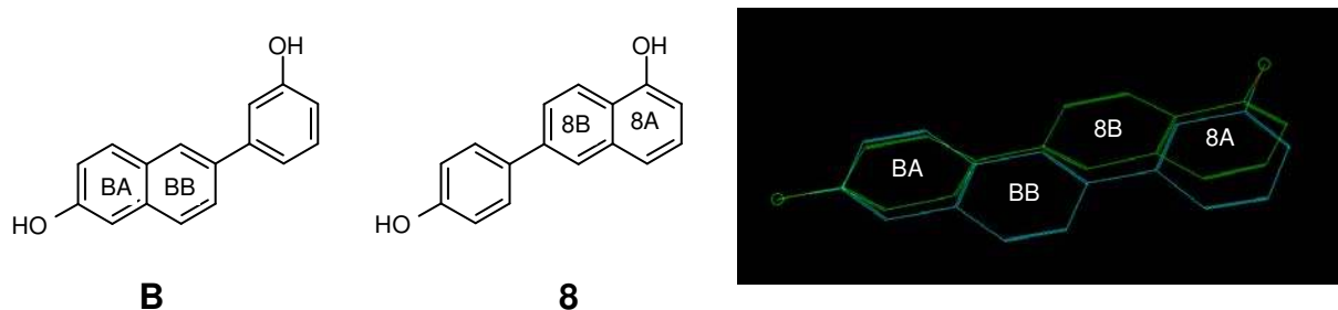
Chart 3. Superimposition of compounds B and 8 .
