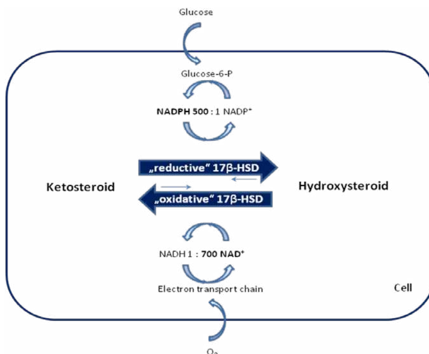
Figure 3: Interplay between metabolism and 17\beta -HSD reactions
