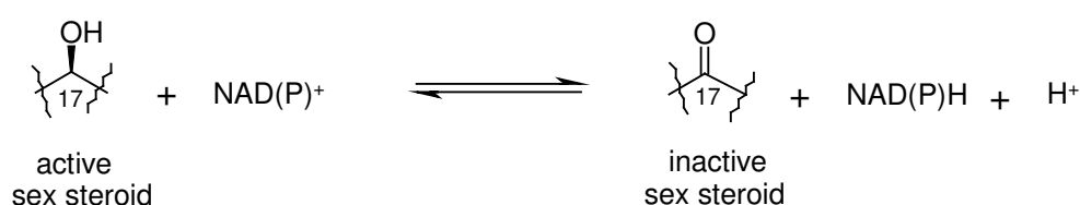
Figure 2: General pathway of reactions catalysed by 17β-HSDs
