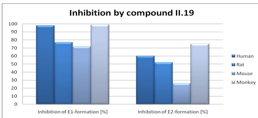
Figure 15: Inhibition of E1- and E2-formation by compound II.19 in different species at 1 \mu M
