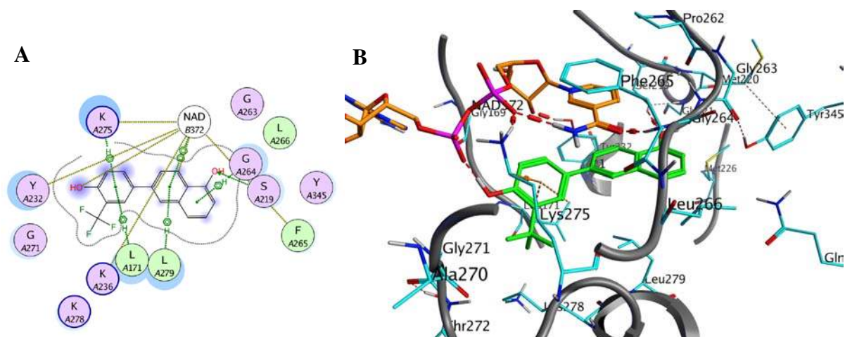
Figure 18: (A) Schematic representation and (B) homology model of compound II.19 (partial mixed inhibitor) in the active site of 17 \beta -HSD2
