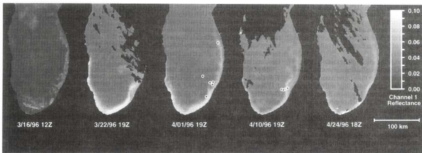
Fig. 1. Visible band satellite imagery of southern Lake Michigan. On March 16, the NOAA 12 (morning) AVHRR Channel 1 satellite image shows shore-fast ice along the eastern shore of the southern basin and large ice floes at the south end of the lake. After several days of warming temperatures and strong northerly winds, the March 22 NOAA 14 (afternoon) image shows the presence of a highly reflective plume that appears to originate along the southwestern shoreline and extend eastward along the southern shore. On April 1, a helicopter was used to collect five samples from the plume region and one sample and two conductivity-temperature-depth profiles were collected from ship further north. A subsequent set of four samples and conductivity-temperature-depth profiles were collected by small boat on April 10. Sampling locations are marked by crosses. By April 24, the plume extended along the entire eastern shore, but the intensity was considerably diminished. The majority of the western shoreline is composed of silty-clay bluffs [Jibson et al., 1994], while the southern shore is highly industrialized with extensive man-made features. The eastern shore is primarily sandy beaches backed by dunes. The pattern of sediment accumulation is highly asymmetric; the western and southern regions do not accumulate recent sediments, while the highest sediment accumulation in the lake is on the southeastern slope (coincident with the eddy features in the figure) and not in the deep central region. Clouds are masked out on the March 22, April 10, and April 24 images.
