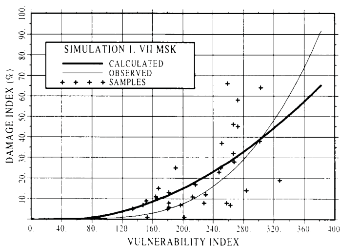
Fig. 8 Simulated (thick line) and observed (thin line) vulnerability functions for MSK intensity VII (Barbat et al., 1996)
