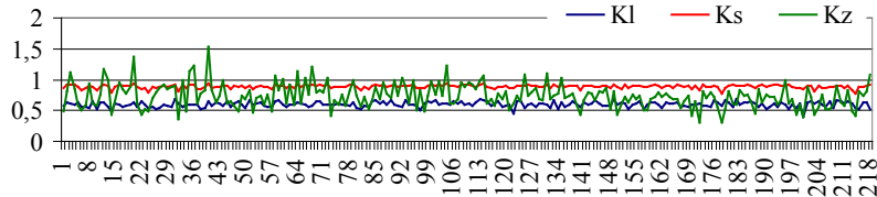
Fig. 4. Comparison of distribution of speech coefficients K_l , K_s and K_z
