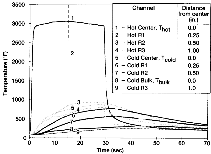
Figure 6.—Temperature rise vs. time for simulated hot gas exposure showing upstream (hot) and downstream (cold) temperatures for Carbon-3. Left hand temperatures removed for clarity.
