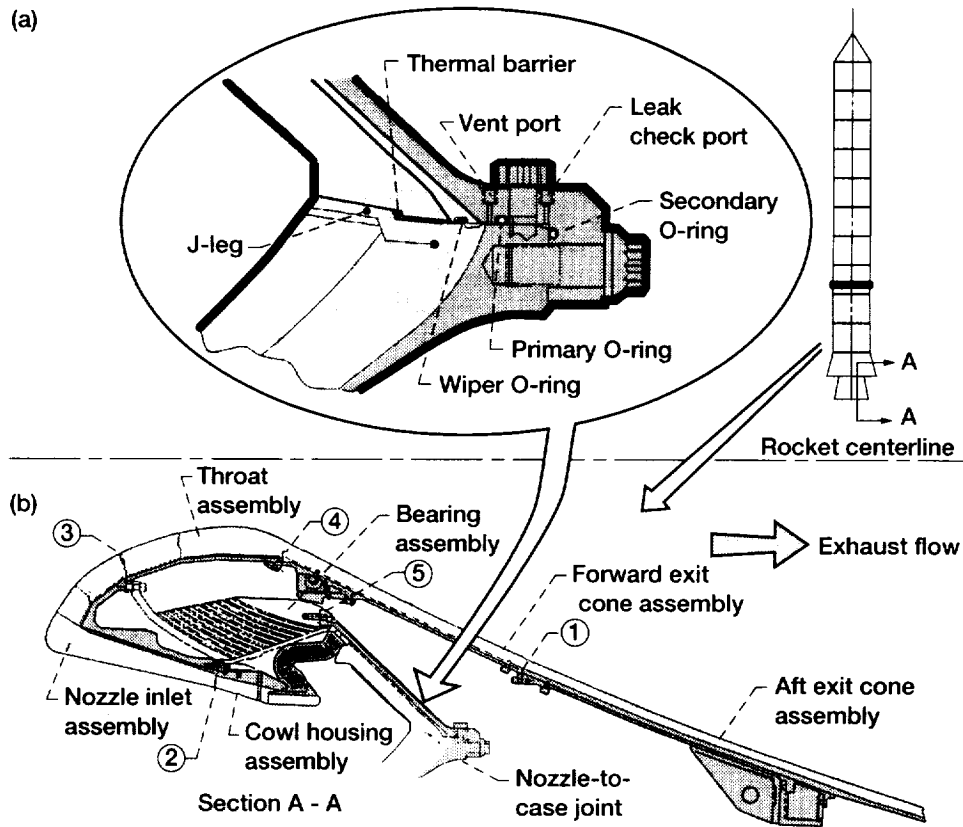
Figure 1.—Potential Shuttle solid rocket motor joint locations for thermal barrier. (a) Enlarged view of nozzle-to-case joint showing J-leg, wiper, primary, and secondary O-rings, leak-check port, and proposed thermal barrier location. (b) Overall nozzle cross-section (half view).
