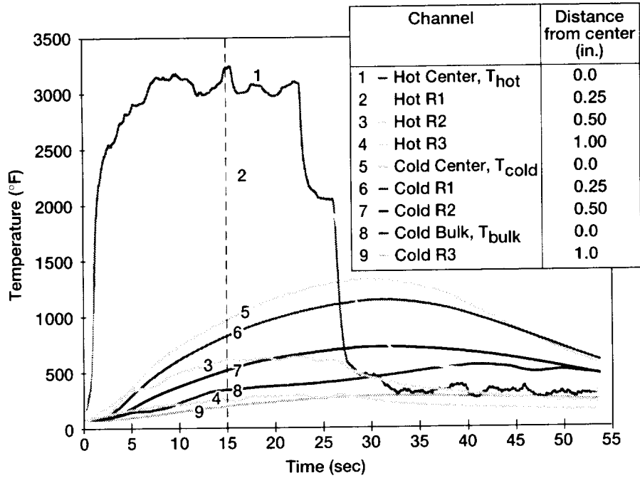
Figure 7.—Temperature rise vs. time for simulated hot gas exposure showing upstream (hot) and downstream (cold) temperatures for Carbon-6. Left hand temperatures removed for clarity.
