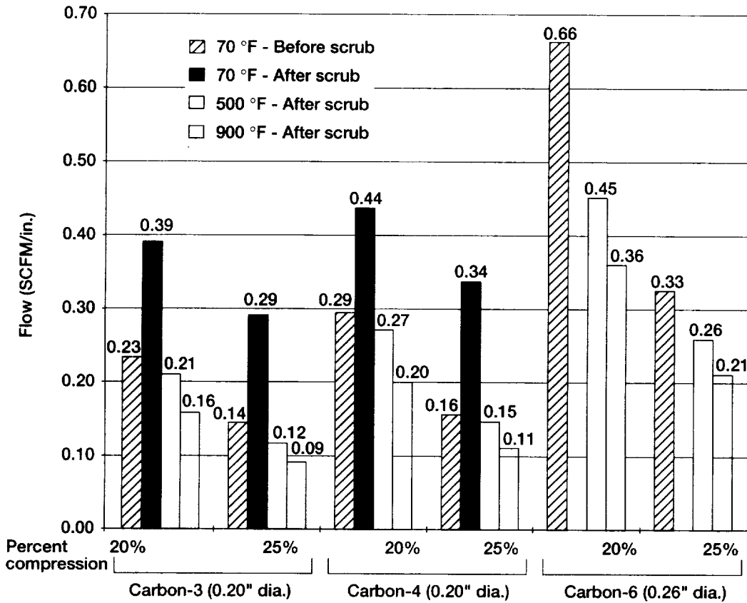
Figure 11.—The effect of temperature, thermal barrier type, scrubbing and compression on flow, \Delta P = 60 psid.
