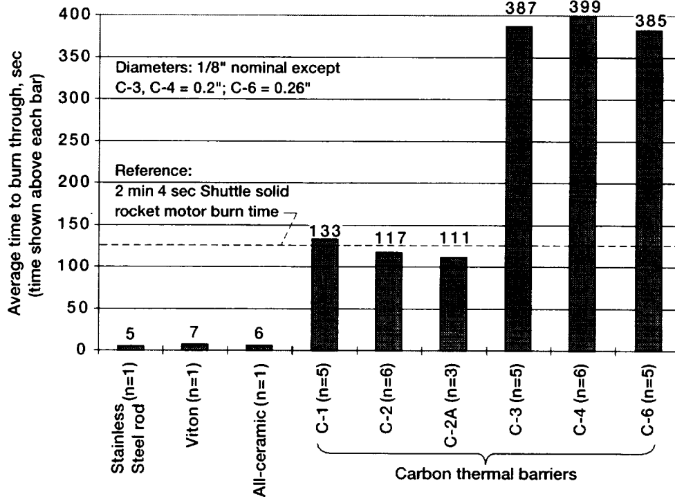
Figure 5.—Oxyacetylene torch burn test results (n = number of tests performed).
