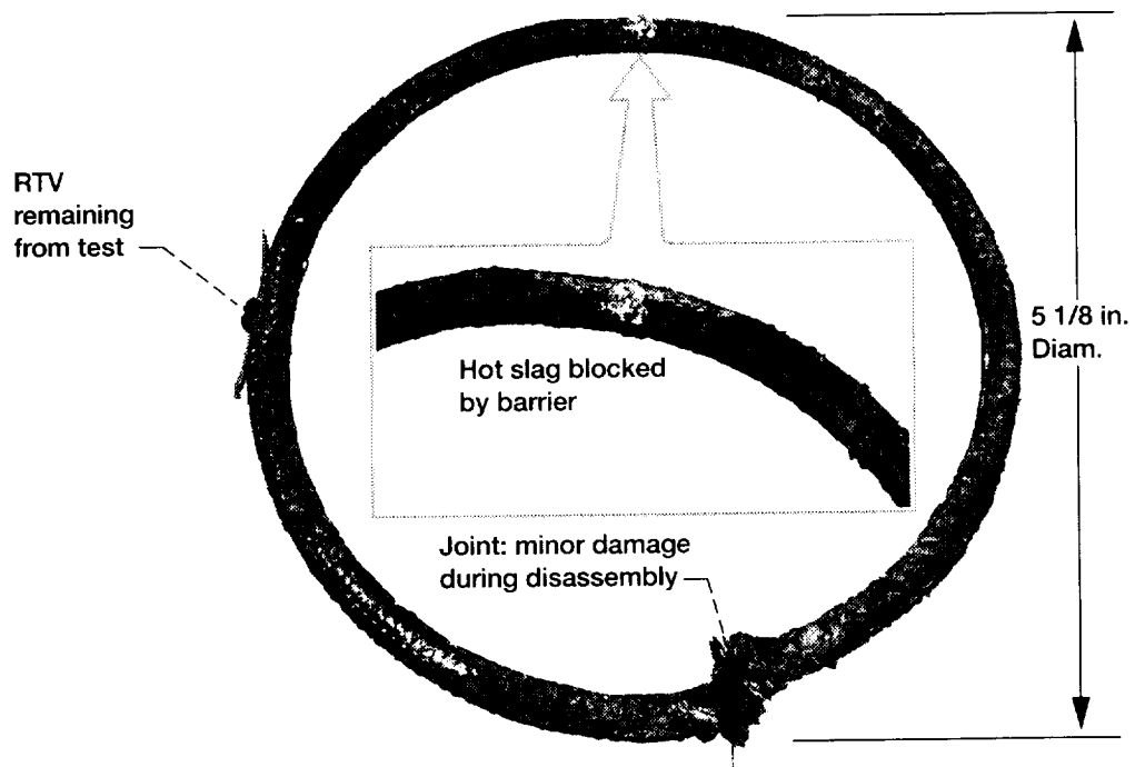
Figure 13.—Photograph of char motor thermal barrier (Carbon-6) after test. Thermal barrier effectively blocks 3200 °F gas for 11 sec. (joint fill time) and blocks hot slag. (Courtesy of Thiokol Corp.)
