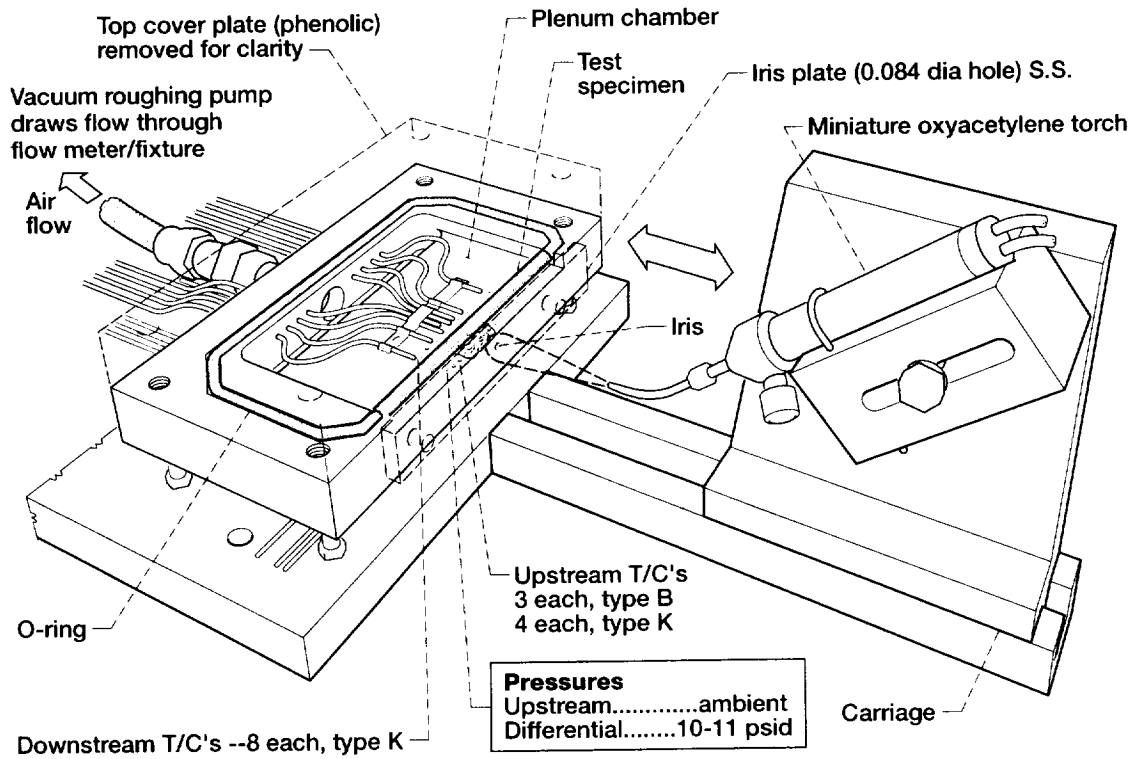
Figure 2.—Schematic of temperature drop test fixture.
