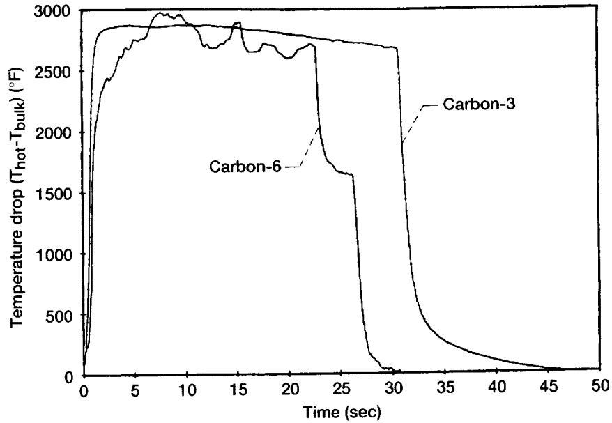
Figure 8.—Temperature drop vs. time ( T_{hot}-T_{bulk} ) at flame location for Carbon-3 and Carbon-6.
