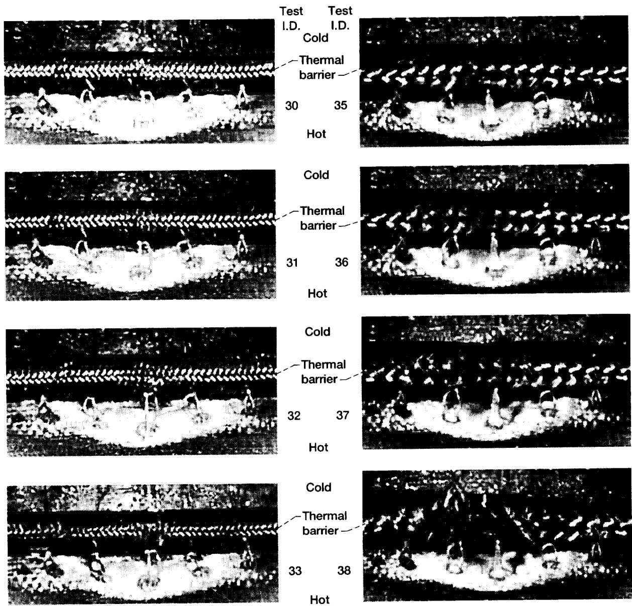
(b) Carbon-6 Temperature Drop Test Results
