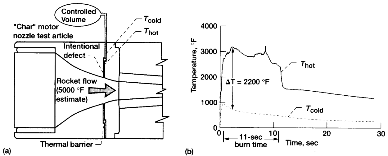
Figure 12.—Subscale (70 lbm) "char" motor tests examining thermal barrier (Carbon-6) effectiveness. (a) Test configuration: Carbon-6 thermal barrier impedes hot gas flow through intentional joint defect (0.06 in. gap). (b) Temperature data: Upstream ( T_{hot} ) and downstream ( T_{cold} ) sides of thermal barrier. (Courtesy of Thiokol Corp.)
