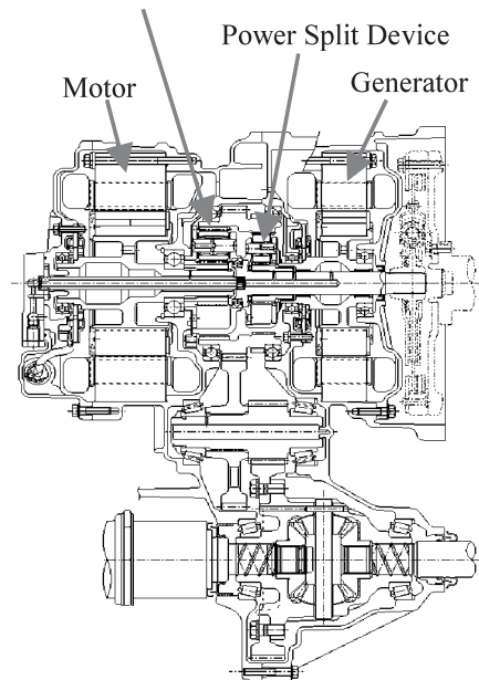
Fig. 4. Cross sectional view of THS II
