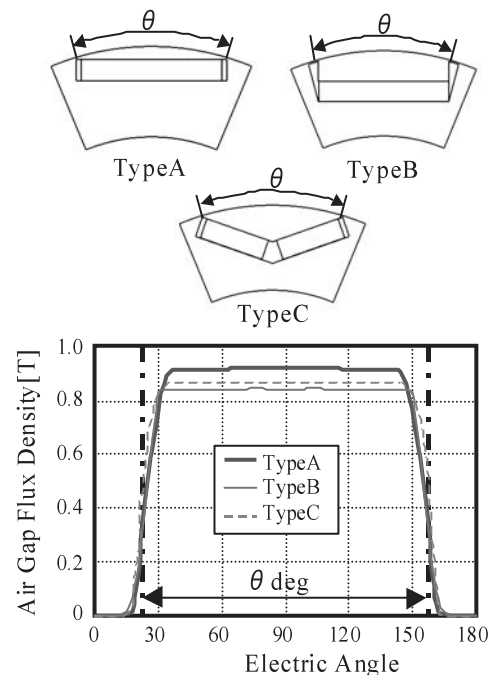
Fig. 10. Air gap magnet flux distribution
