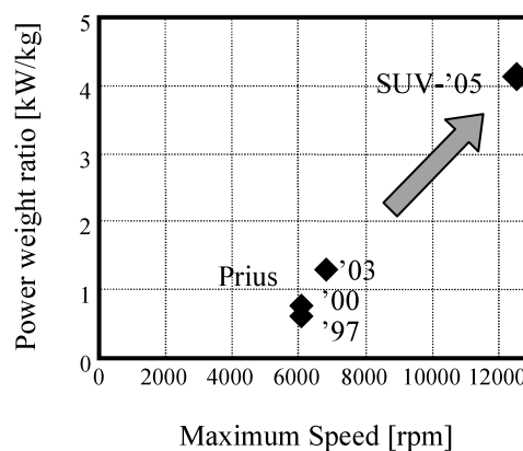
Fig. 1. Historical diagram of Power weight ratio improvements in the THS traction drive motor
