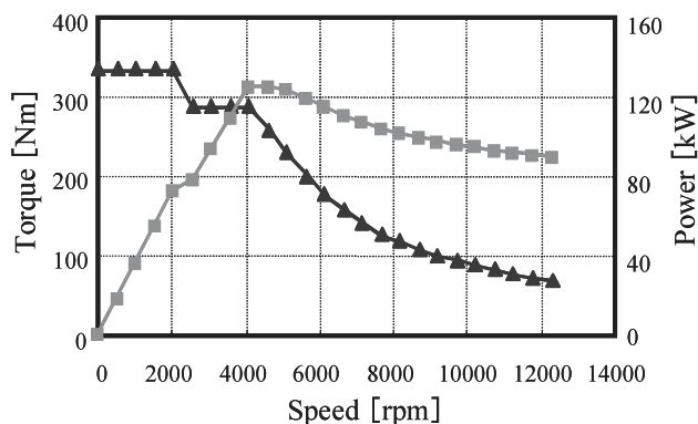
Fig. 14. Power/torque characteristics of newly developed motor
