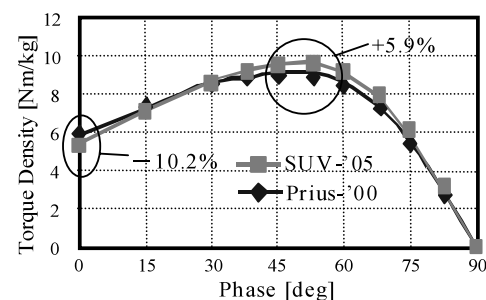
Fig. 3. Torque phase characteristics
