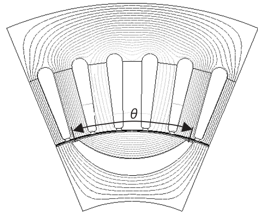
Fig. 9. Vector potential contour lines and \theta
