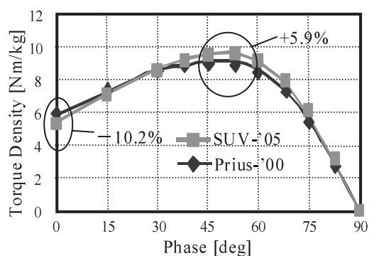
Fig. 15. Torque phase characteristics
