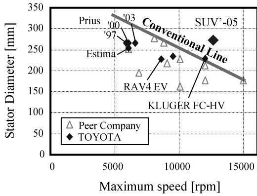
Fig. 6. Relationship between stator outer diameter and maximum speed of recently developed motors for EVs and HEVs
