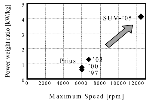
Fig. 1. Historical diagram of Power weight ratio improvements in the THS traction drive motor
