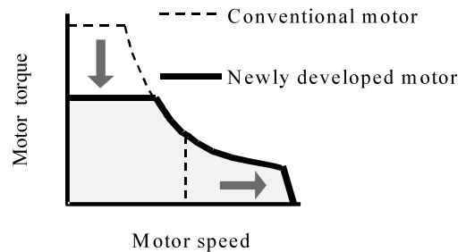
Fig. 2. Motor down sizing by reduction gear
