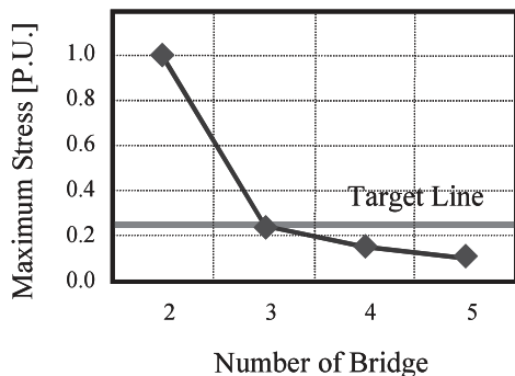
Fig. 12. Bridge quantity and stress
