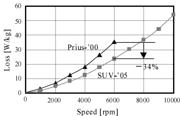
Fig. 17. Measured no-load loss
