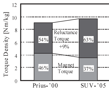
Fig. 16. Torque ratio comparison
