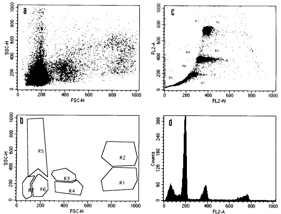
FIG. 1. FACS analysis of a testicular cell suspension obtained from an adult mouse. a ) First window, in which cells are distributed according to size (FSC-H) and cellular granularity (SSC-H). b ) The frame of the first window overlaid with marks representing the seven gated groups. Marks are not shown on original plot to enable better discrimination of the groups mentioned. c ) Second window, in which cells are distributed according to fluorescence intensity (FL2-A) and width of the emitted fluorescence (FL2-W). Location of gated groups is marked by their group number (R1-R7). d ) A histogram that represents the number of cells at each fluorescence level.
