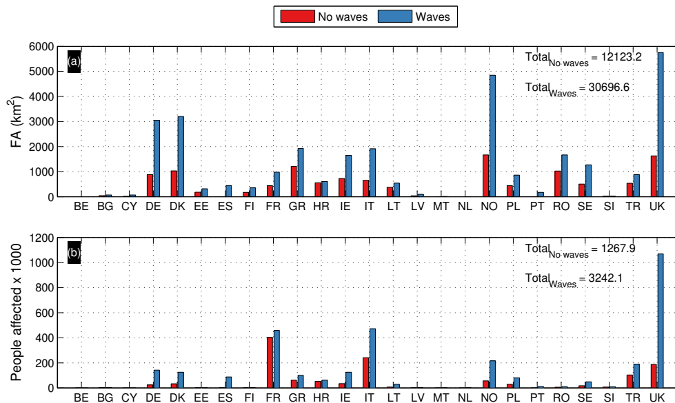
Figure 9. Estimated values of the country level FA (a) and thousands of people affected (b) for the present-day 100-year event; comparisons between the results considering TWLs including/excluding waves.
