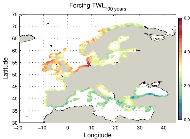
Figure 1. Total water level values for the present-day 100-year event along the European coastline; values are shown every 25 km of coastline.
