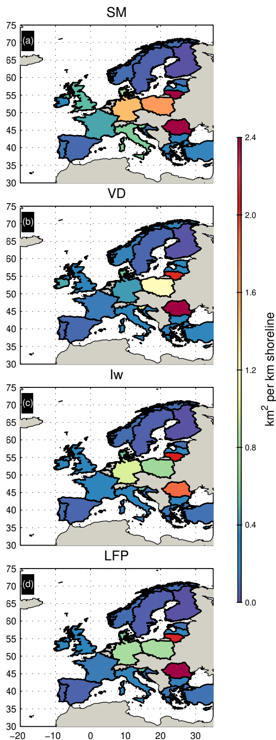
Figure 6. Estimated coastal flood extent for the present-day 100-year event using all four approaches, aggregated per country level, and normalized by coastline length. Values correspond to km 2 per km of coastline.
