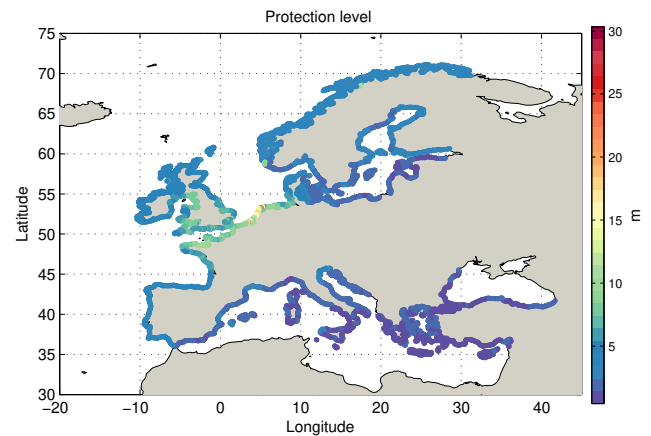
Figure 2. Protection standards considered along the European coastline, expressed as design total water levels (TWLs).
