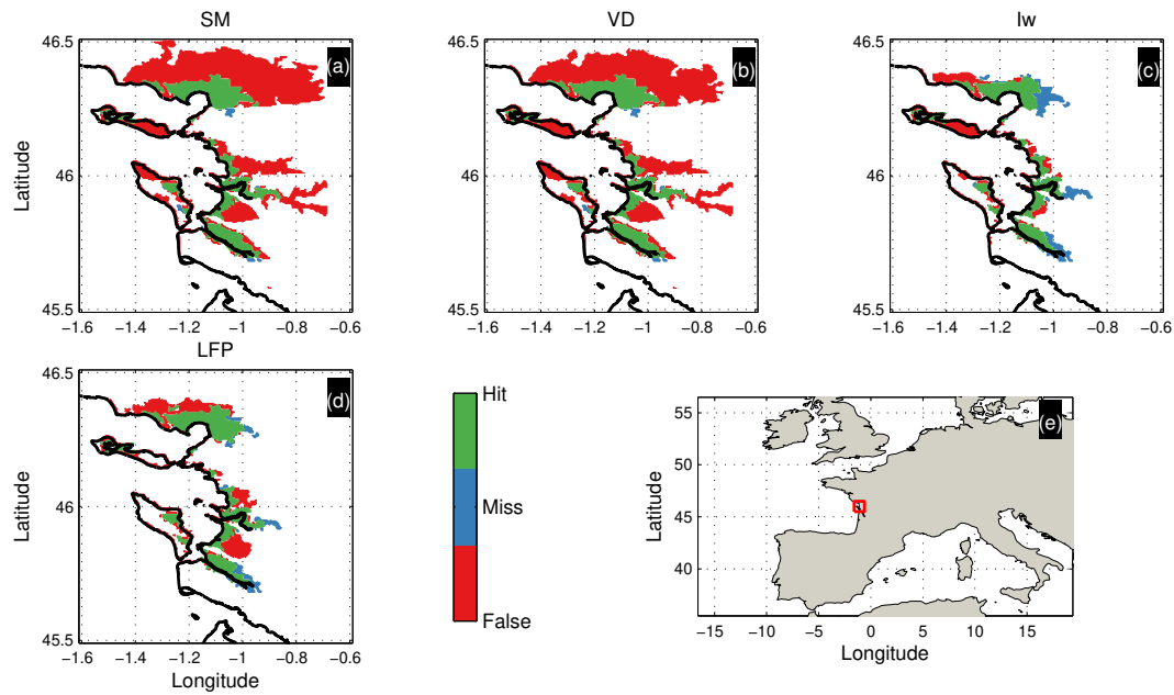
Figure 3. Validation of the LISFLOOD-FP model for the Xynthia storm: maps showing the comparison of the simulated and observed flood extent, as well as their intersection: green, blue and red colors correspond to inundated areas predicted, not predicted and overpredicted by the model, respectively. Map (e) shows the location of the study area.
