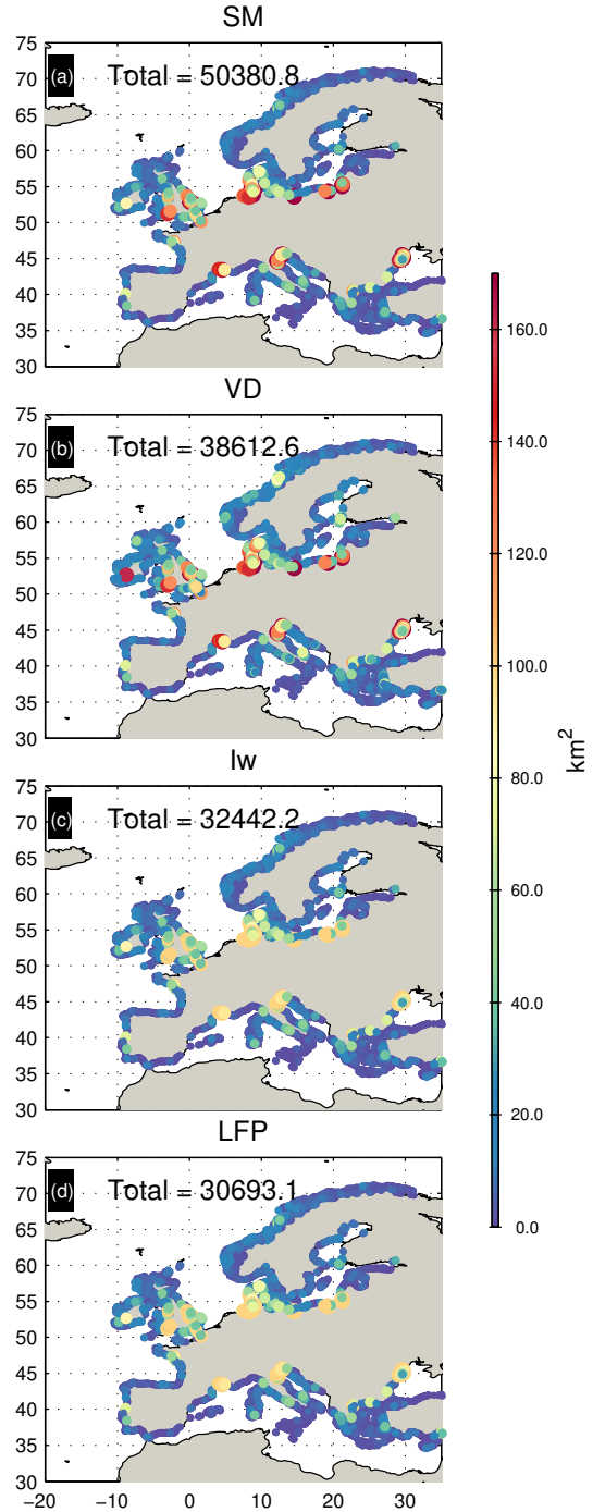
Figure 5. Estimated coastal flood extent for the present-day 100-year event using all four approaches. Values are shown for each 25 km coastal segment and correspond to km 2 .
