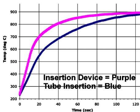
FIG. 6. (Color online) Plot of time in seconds vs temperature in degrees centigrade, which shows the time from 230 °C (temp in-tube preinsertion) to 900 °C (SWCNT synthesis temperature) for the silicon sample. Note that the time to reach 860 °C (the temperature at which growth is initiated by introducing methane into the chamber) is 66.5 s for the insertion device, and 105 s for the alternative approach of sliding the tube into the furnace.
