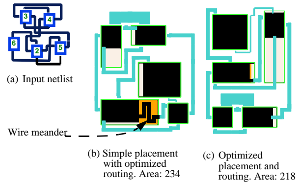
Fig. 7. Impact of length constraints on optimization
