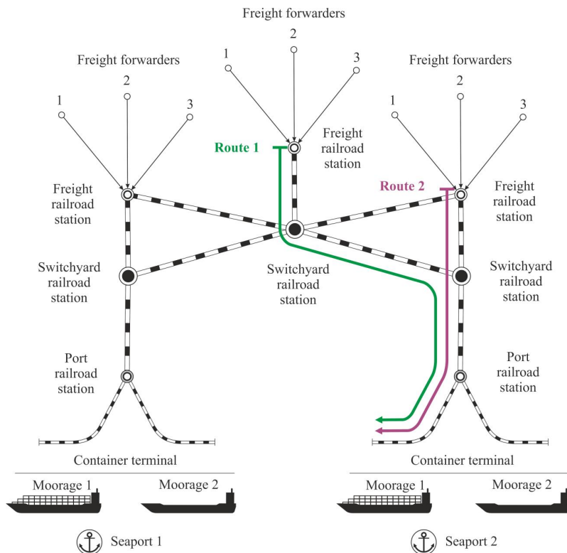
Fig. 1. The scheme of organization of delivery of containers by railroad to seaports in intermodal transportation
