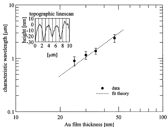
FIG. 4. Dependence of the characteristic wavelength of the surface modulations on Au film thickness. The fit is based on the dependence predicted by the theory of spinodal dewetting. The inset shows a topographic linescan of the surface modulations at a 47 nm thick Au film, as it can be extracted from the SNAM measurements.
