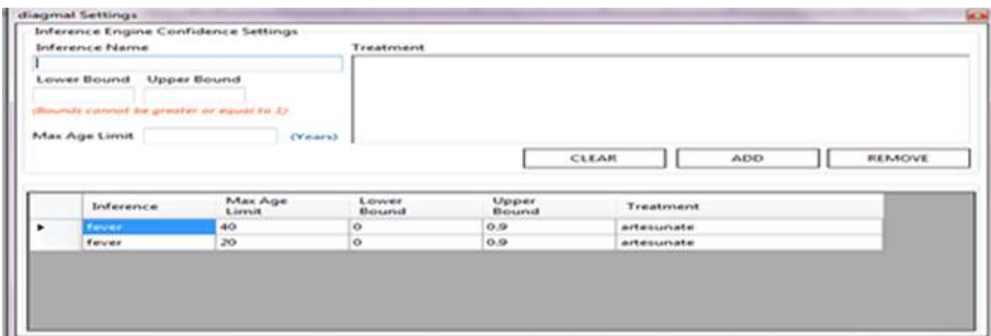
Fig. 7. Inference result
