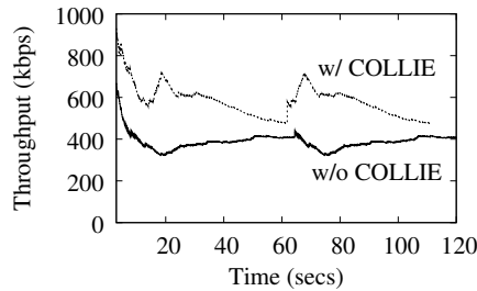
Fig. 15. Observed throughput for mobile scenario
