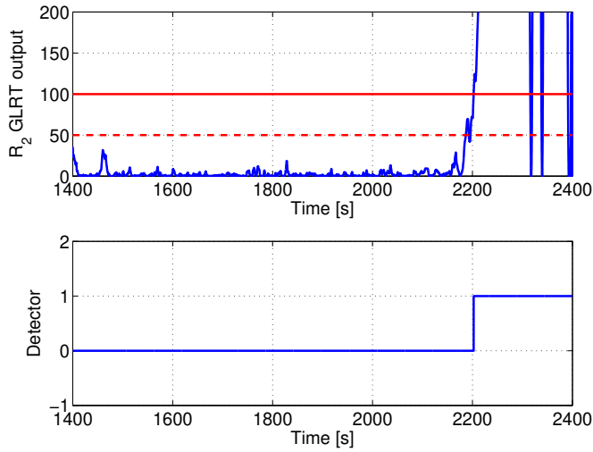
Fig. 15. GLRT output and decision signal from R_2 . The alarm is raised at t = 2202 s. The solid horizontal line is the threshold for alarms and the dashed line is the threshold for stopping estimation.
