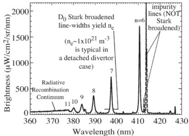
Fig. 24. Measured visible spectrum of the high- n D Balmer series from a detached divertor plasma. Evident are the Stark-broadened Balmer lines, their intensity decrease according to a Saha-Boltzmann population of the upper levels and the radiative recombination continuum ( \lambda < 370 nm).
