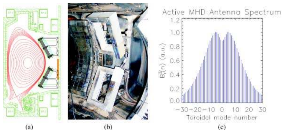
Fig. 32. (a) Poloidal cross section of C-Mod showing the locations of the two active MHD antennas relative to the outboard limiter and a typical plasma equilibrium, (b) photo of the active MHD antennas in C-Mod, and (c) calculated active MHD antenna toroidal mode spectrum with a FWHM of |n| \sim 16 .
