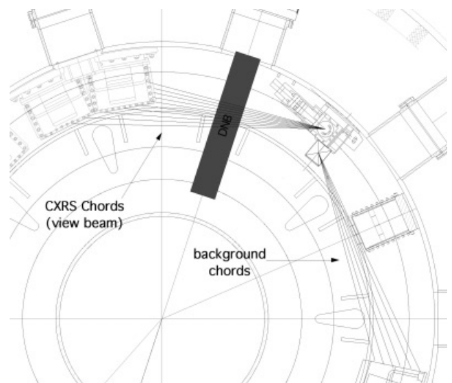
Fig. 11. Location of the toroidal CXRS views during the 2004 and 2005 campaigns. One views the beam and the other views plasma without the beam to use for background subtraction in the event of low CXRS signal levels.
