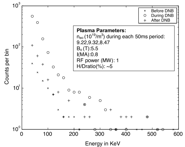
Fig. 30. CNPA signal during low-density L-mode C-Mod discharge 1040415006. The three sets of data shown are counts from 50 ms before, during, and after the DNB fires. Clearly, the DNB increases the CNPA signal significantly.
