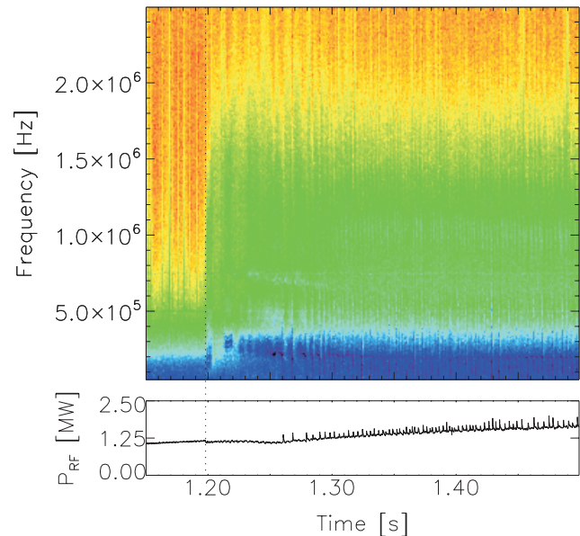
Fig. 17. Top: Spectrogram of a core PCI channel. The color scale is logarithmic (dark blue is high amplitude, red is low amplitude), the time resolution is 1 ms, and the frequency resolution is 5 kHz. The vertical dashed line marks the transition from L-mode to ELMY H-mode. Bottom: Trace of ICRF power.
