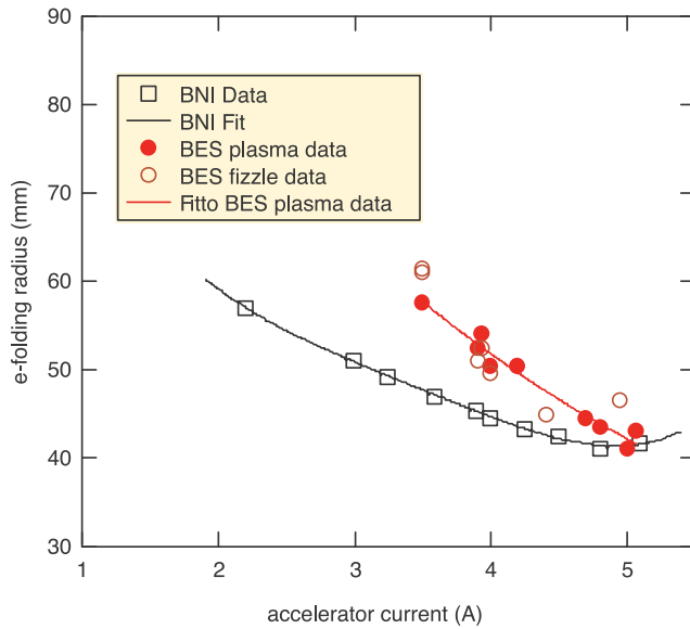
Fig. 9. DNB e-folding radii versus beam current from specifications (black squares and line) and measured by BES (circles and line [red online]). The black points were measured using calorimetry while BES measured emission from only the full-energy beam component.
