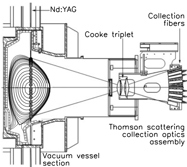
Fig. 3. Cross section of the C-Mod vacuum vessel with contours of constant poloidal flux for a sample plasma discharge. The TS collection optics is mounted such that a Nd:YAG laser beam passing along a vertical chord through the plasma is imaged onto a set of optical fibers. Circles along the beam path represent scattering volumes.
