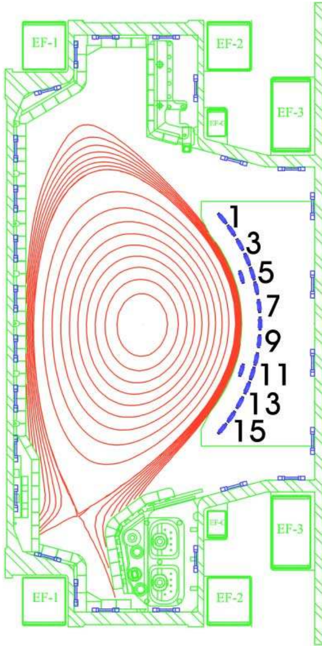
Fig. 15. Cross section of C-Mod showing the magnetic pickup coils (blue online) on one side of the full limiter and the main magnetic diagnostics (blue online) in the GH sector.
