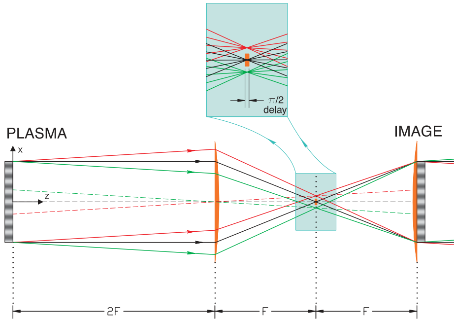
Fig. 16. Schematic drawing illustrating the PCI technique.
