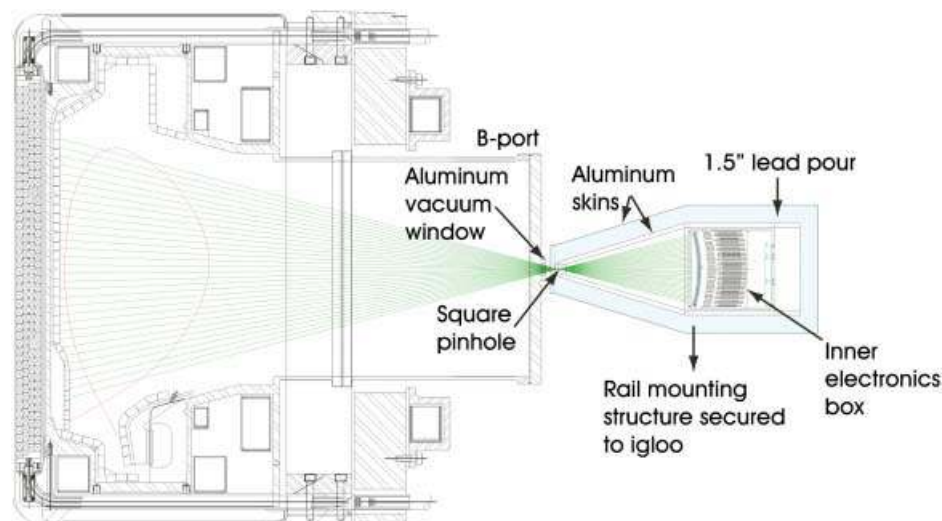
Fig. 31. Setup of the hard X-ray camera.
