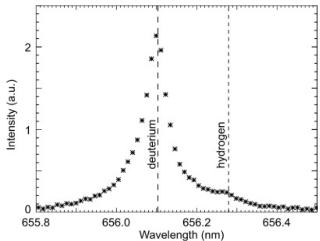
Fig. 28. Typical H/D Balmer- \alpha spectrum, showing the locations of the D (majority) and H (minority) peaks.
