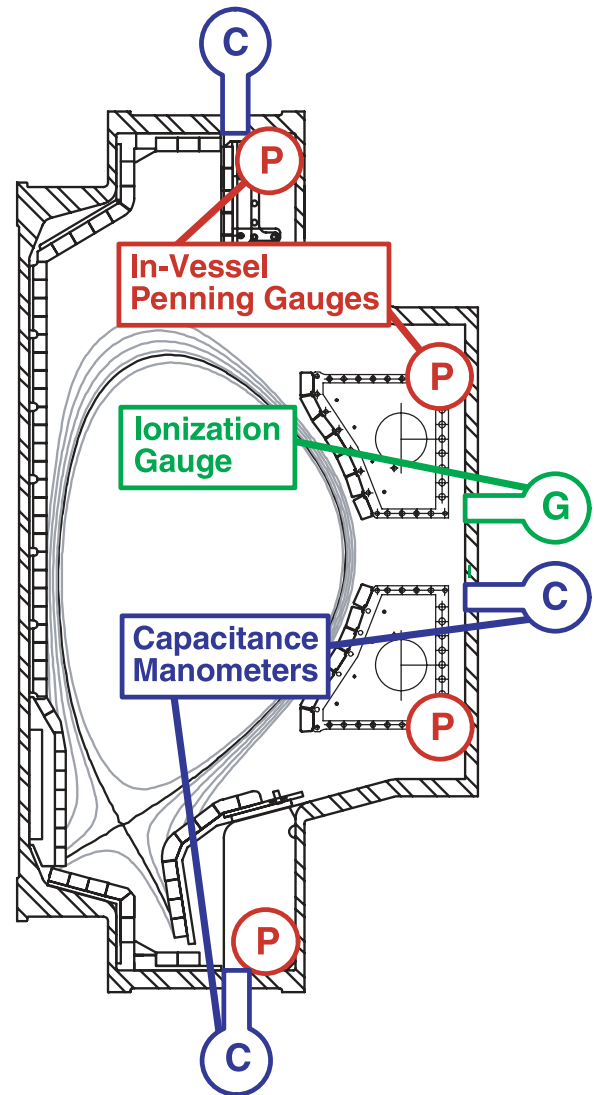
Fig. 1. Three types of gauges are used to monitor gas pressure in the divertor and main chamber regions of C-Mod. These include cold cathode Penning ionization gauges mounted on the wall of the vacuum vessel (P), absolutely calibrated capacitance manometer gauges (C), and Bayard-Alpert-type ionization gauges (G). Gauges C and G are magnetically shielded and located outside the influence of the toroidal magnetic field at the ends of diagnostic ports. The Penning gauges use the intrinsic magnetic field for operation and are an adaptation of a commercially available unit.
