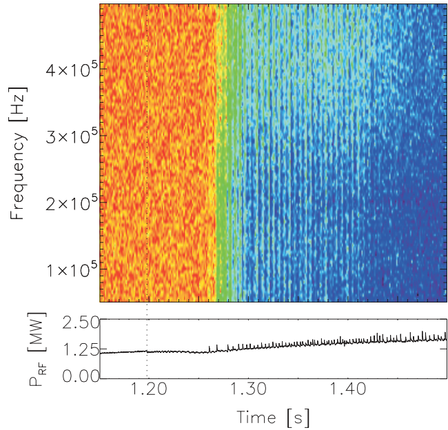
Fig. 20. Top: Spectrogram of the 132-GHz reflectometer channel. The color scale is logarithmic (dark blue is high amplitude, red is low amplitude), the time resolution is 1 ms, and the frequency resolution is 5 kHz. The vertical dashed line marks the transition from L-mode to ELMy H-mode. Bottom: Trace of ICRF power.
