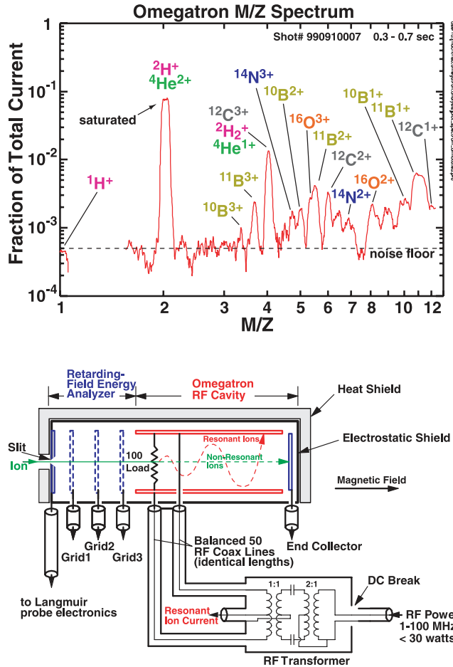
Fig. 27. Typical M/Z ion spectrum from the omegatron probe (top) and arrangement of grids and rf cavity (bottom).
