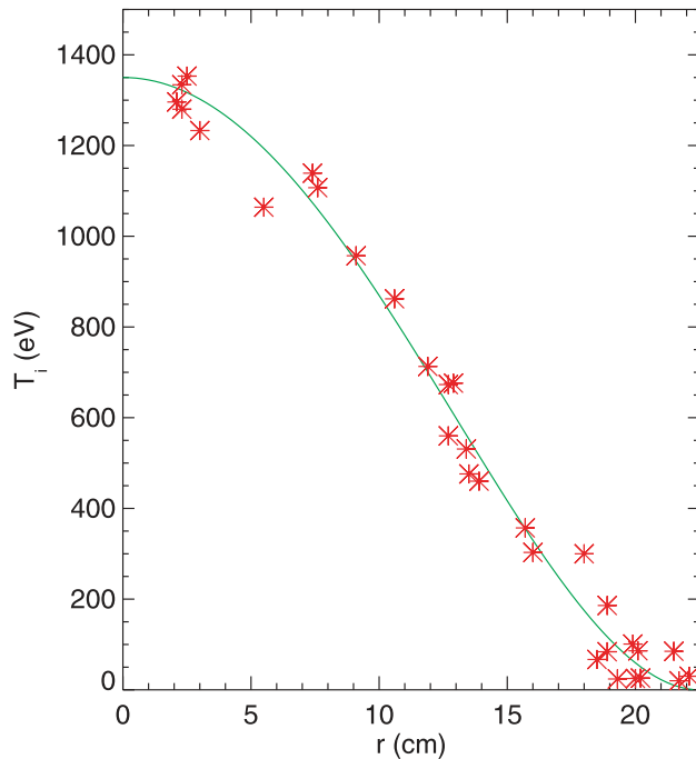
Fig. 7. Ion temperature profile for an L-mode discharge. The asterisks are the measurements and the line is an analytic fit to the data.
