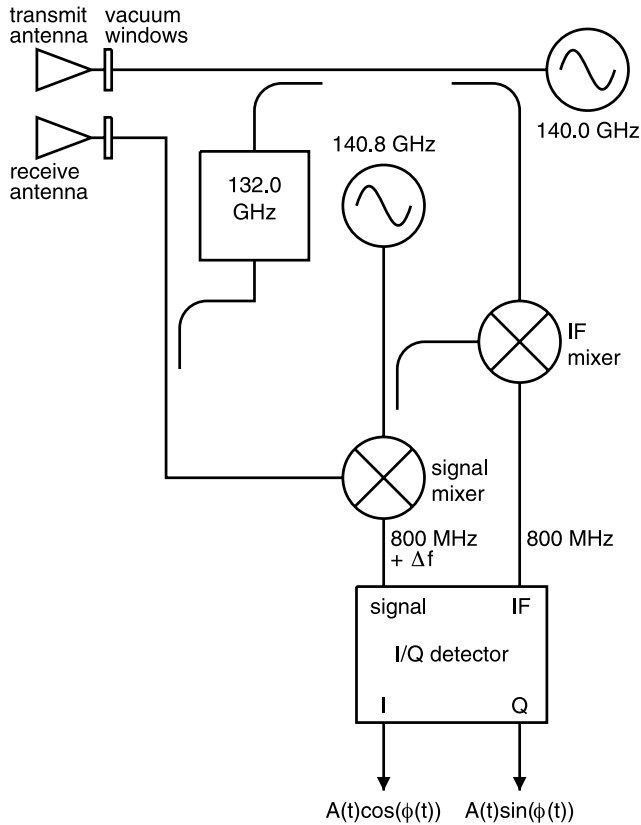
Fig. 19. Layout of the high-frequency millimeter wave system of the reflectometer.
