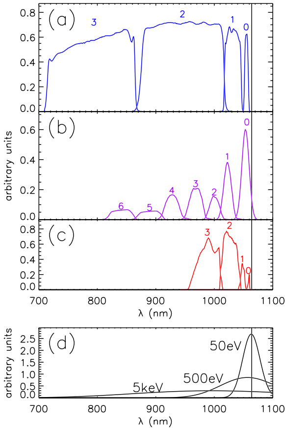
Fig. 4. Typical spectral responses of (a) the core TS upgrade polychromators, (b) the original core spectrometers, and (c) the edge TS polychromator. The vertical line at \sim 1064 nm represents the Nd:YAG laser line. (d) TS spectral distribution for a given n_e at three values of T_e .
