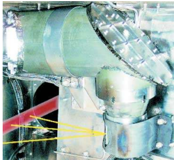
Fig. 13. The MSE/BES in-vessel optical periscope. An artist's conception of the DNB (smaller than actual) and example view chords are indicated in red and yellow, respectively. The light is reflected upward by a mirror behind the entry lens through two additional lenses to another mirror (attached to the ribbed oval plate at the upper right-hand side of the photo). This mirror reflects the light toward the left to a third mirror (the bright plate at the upper left-hand side of the photo), which relays the light out of the vessel.
