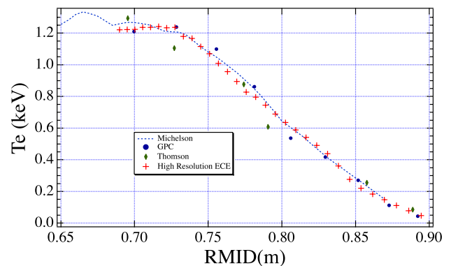
Fig. 2. T_e profiles from ECE diagnostics (Michelson, GPC, and high-resolution ECE) and Thomson scattering for a typical 5.4-T C-Mod discharge.
