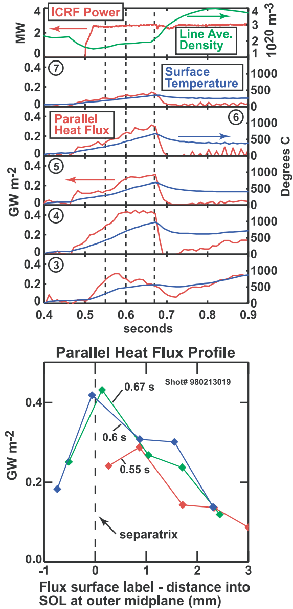
Fig. 26. Data traces from divertor heat flux probes (top) and resultant parallel heat flux profiles at three times in the discharge (bottom). Circled numbers indicate probe locations on the divertor (see Fig. 25).
