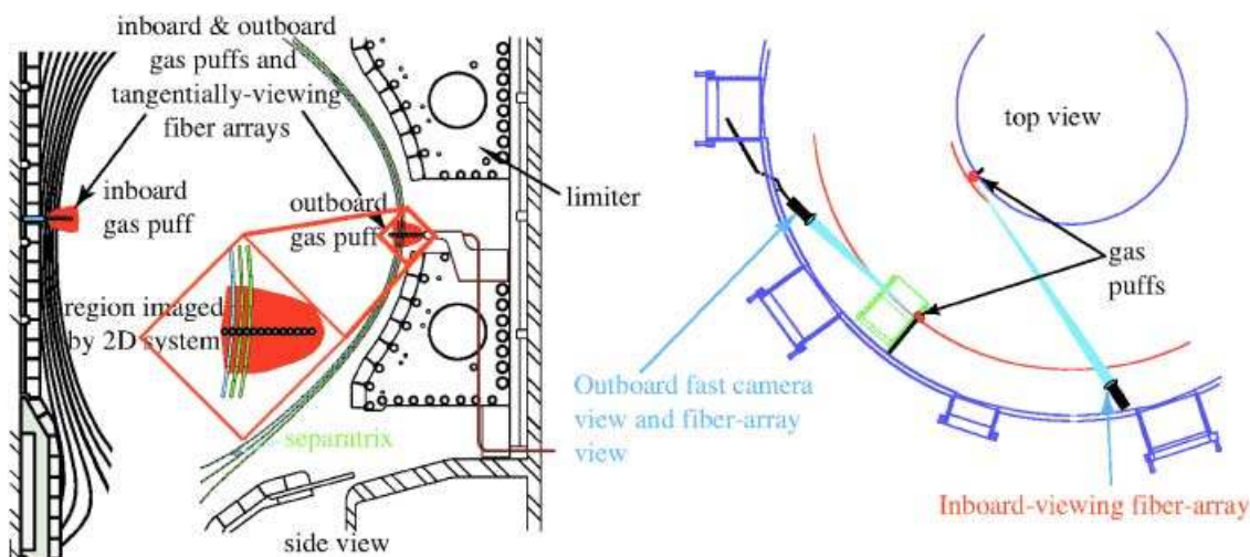
Fig. 23. Schematic of the GPI systems (side and top views).
