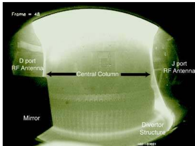
Fig. 21. Radially inward view from one of the survey cameras. The in-vessel hardware is as labeled.
