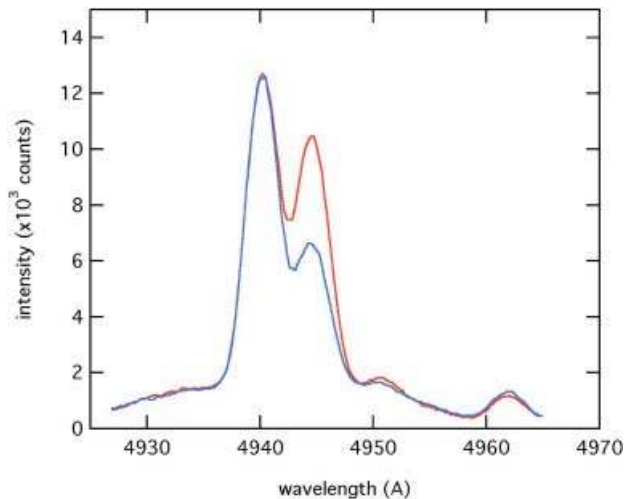
Fig. 12. The line used to detect CXRS emission is 4944.67 Å ( n = 7 \rightarrow 6 ) \text{B}^{+4} . It is blended with a line from a lower ionization stage, 4940.376 Å, 2s3d^1D_2 - 2s4f^1F_3\text{B}^{+1} . One spectrum (red) is taken during a beam pulse. The other (blue) is taken just after the beam pulse.
