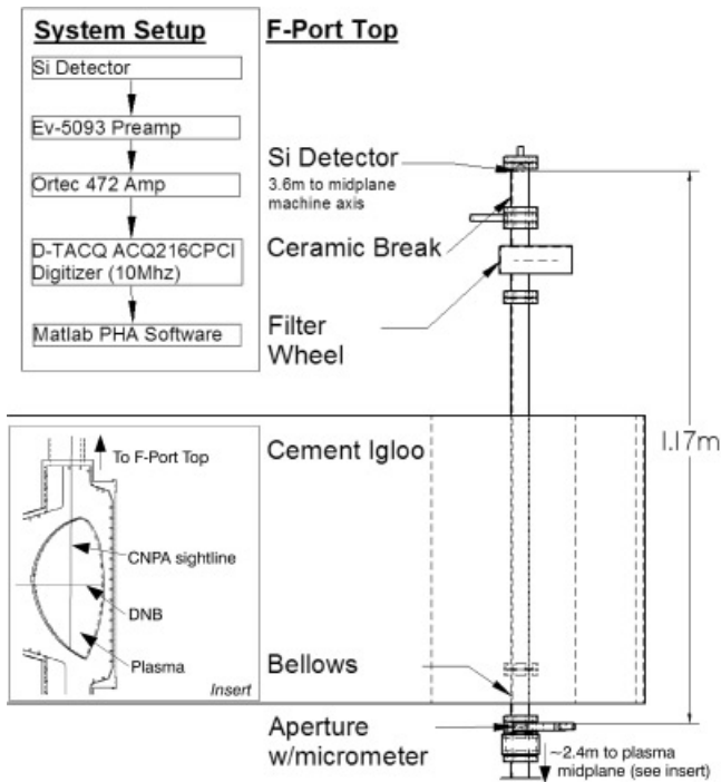
Fig. 29. CNPA schematic during the spring 2004 campaign.
