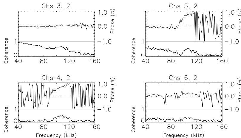
Fig. 14. Coherence and phase between various BES views at R = 88.5 \text{ cm} . Channels 3, 4, 5, and 6 are separated vertically from channel 2 by 0.0, -4.5 , -1.5 , and +3.0 \text{ cm} , respectively. The feature at 100 to 120 kHz is the quasi-coherent mode.
