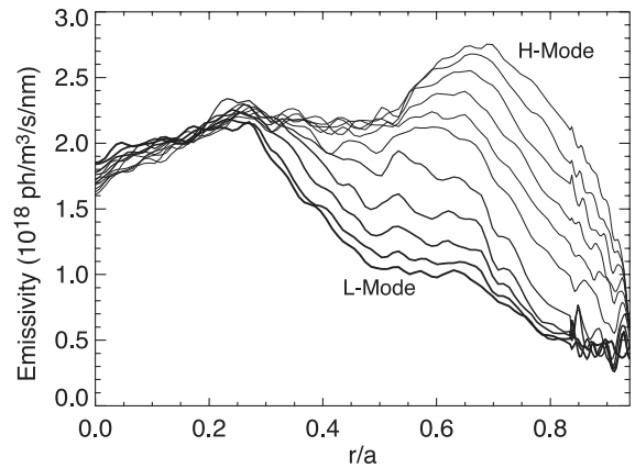
Fig. 6. Visible continuum emissivity profile evolution following an H- to L-mode transition after ICRF heating is turned off in a C-Mod discharge. The profiles, which are plotted at 2-ms intervals, show the evolution that results from the loss of the ETB, leading to a progressive decay of density that propagates inward from the plasma boundary. The traces become bolder as time progresses.
