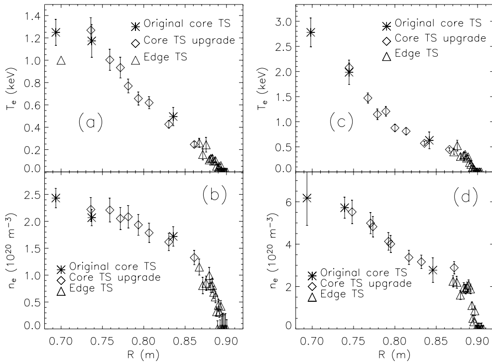
Fig. 5. Typical T_e and n_e profiles in different plasma regimes. Only three spatial channels were working in the original core TS system for this plasma discharge. (a) T_e and (b) n_e profiles during an L-mode discharge. (c) T_e profile in H-mode, exhibiting a clear H-mode pedestal. (d) n_e profile in a double-barrier regime, where an ITB forms in the presence of an H-mode pedestal at the edge. Good agreement between all three C-Mod TS diagnostics is observed for all plasma regimes.
