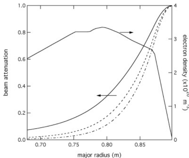
Fig. 10. Simulation of the beam penetration into an EDA H-mode discharge (1031209028 at 1 s). The attenuation of the beam components at the beam energy (solid line), one-half the beam energy (dashed line), and one-third of the beam energy (dotted-dashed line) are shown. A density profile is also displayed.
