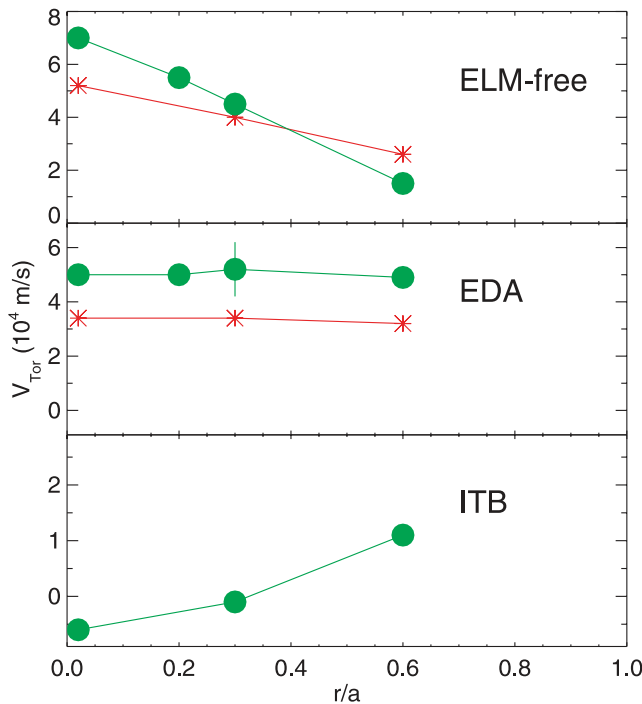
Fig. 8. A comparison of toroidal rotation velocity profiles in two different edge-localized-mode-free H-mode plasmas (top), two different EDA H-mode discharges (middle), and an ITB plasma (bottom).
