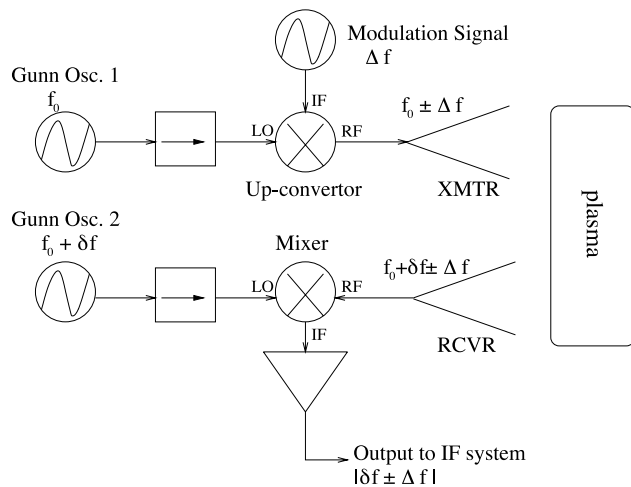
Fig. 18. Layout of the low-frequency millimeter wave system of the reflectometer.
