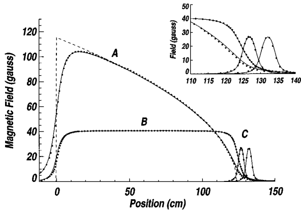
FIG. 2. Plot of the measured spatial dependence of the magnetic fields at a current of 1 A through all windings (dots). The labels A, B, and C indicate the profile, bias, and extraction coils, respectively. The solid lines represent the field designs. The dashed line shows the idealized square-root form of the profile magnetic field. The inset shows the magnetic field near the extraction region for the different solenoids.
