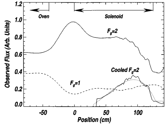
FIG. 11. Atom flux observed at the detector for atoms coming from different positions in the solenoid for both ground hyperfine states. The solid line on the lower right-hand side of the figure represents the measured flux of laser-cooled atoms in the F_g = 2 state. The dotted line is the result of the calculations discussed in the text.
