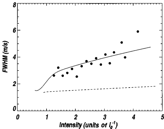
FIG. 6. Intensity dependence of the width of the cold atom peak for the spatially expanded slowing beam. On the horizontal axis the average intensity of the slowing beam is represented. For the calculations we assumed the area intensity function F(s_0) to be Gaussian. The dashed curve gives the calculated result for the experimentally determined distribution with rms fluctuations of 5%; the solid line gives a fit to the data, using an intensity distribution function with rms fluctuations of 18%.
