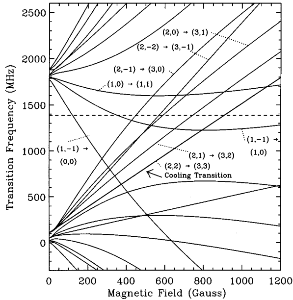
FIG. 8. Plot of optical transition frequencies vs magnetic field for \sigma^+ light. The labels at the lines represent the atomic transitions in the limit for B \rightarrow 0 in the notation (F_g, M_g) \rightarrow (F_e, M_e) . The arrow indicates the cycling transition (F, M_F) = (2, 2) \rightarrow (3, 3) used for slowing. The frequency scale is with respect to the zero-field value of the F_g = 2 \rightarrow F_e = 0 transition. The dashed line indicates the Doppler-shifted frequency of the slowing laser for atoms moving at 700 m/s and a laser frequency tuned 80 MHz above F_g = 2 \rightarrow F_e = 3 . In the rising edge of the magnetic field the atoms first come into resonance with the other m_g \rightarrow M_e transitions originating from F_g = 2 \rightarrow F_e = 3 .
