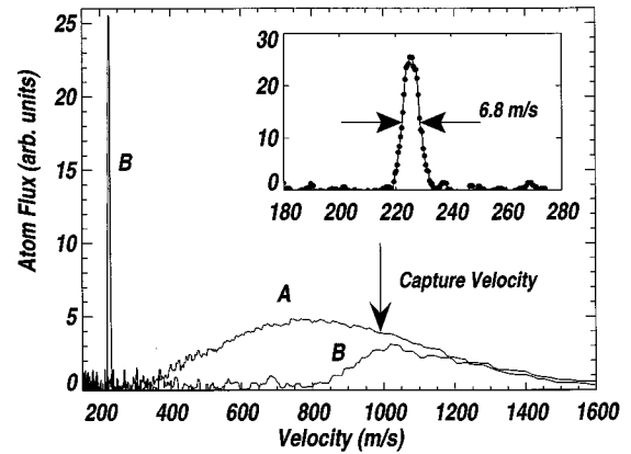
FIG. 3. Measured velocity distributions both with and without the slowing laser beam. The curve labeled A indicates the unsloped distribution from the source. Curve B shows the distribution after slowing. The arrow indicates the maximum of the velocity capture range of the slowing laser. The inset shows an enlarged portion of the figure in which the strong collection of atoms at low velocities is clearly visible.
