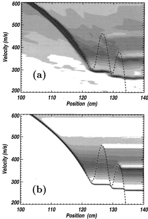
FIG. 10. Contour map of the velocity and position of atoms in the solenoid showing the origin of the multiple peaks structures visible in Fig. 9. (a) shows the measured results and (b) shows the result of the simulations discussed in the text. The dashed lines show the velocity for the atoms in resonance with the cooling transition (F, M_F) = (2, 2) \rightarrow (3, 3) .
