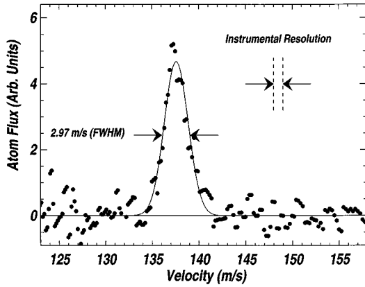
FIG. 5. One of the measured velocity distributions with the flattened laser beam profile. The experimental width of approximately 1/6(\Gamma/k) is shown by the dashed vertical lines between the arrows. The Gaussian fit through the data yields a FWHM of 2.97 m/s.
