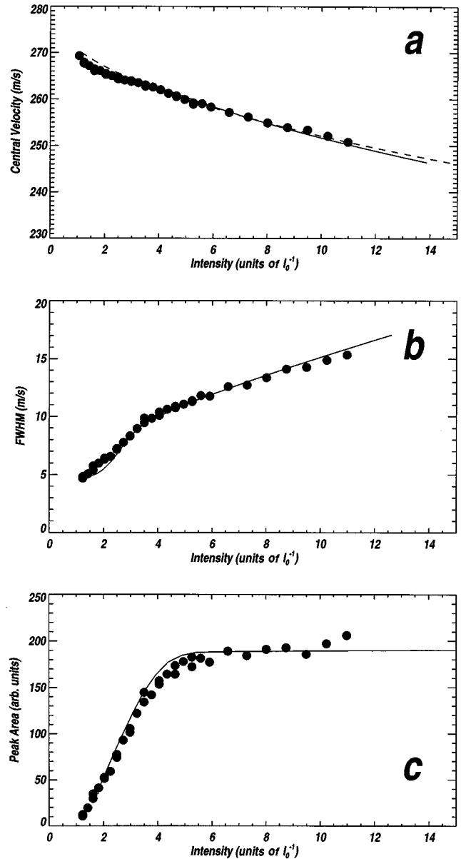
FIG. 4. Intensity dependence for a fixed laser frequency for the three quantities: (a) central velocity, (b) width of the velocity distribution, and (c) the peak area. The dots indicate the measured data points. The solid lines represent the calculated intensity dependence, using a Gaussian slowing beam profile. The dashed line indicates the result of Eq. (6). The intensity is determined at the end of the solenoid and is given in units of the saturation intensity I_0 .
