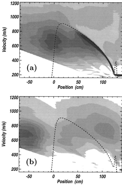
FIG. 7. Contour map of the measured velocity and position of atoms in the solenoid for (a) F_g = 2 atoms and (b) F_g = 1 atoms. The dashed line indicates the resonance frequency for the (F, M_F) = (2, 2) \rightarrow (3, 3) cooling transition. The density of atoms per unit phase-space area \Delta v \Delta z has been indicated with different gray levels.
