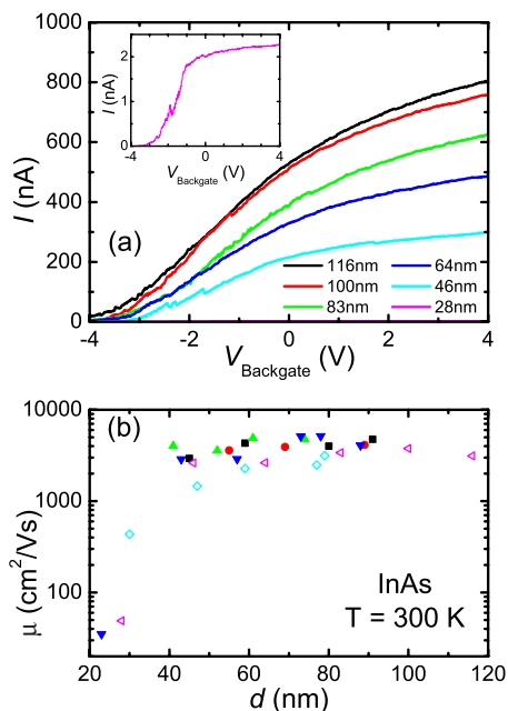
FIG. 3. (Color online) (a) Backgate sweeps for different sections within the same nanowire ( T=300\text{ K} ; same device as in Fig. 1). Applied bias voltage: 10 mV. The inset shows the data for the section with the smallest diameter. (b) Mobility determined from backgate sweeps. Different symbols correspond to the different devices studied, each with several sections of different diameter.
