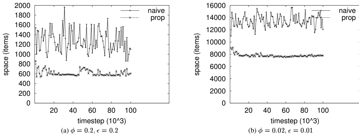
Figure 10: Comparison of data structure sizes from the online algorithms for the overlap case using FLOW with bit-level hierarchies.
