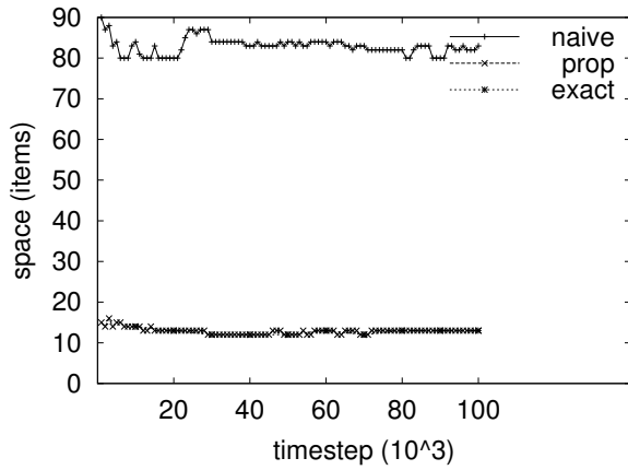
(a) output size
