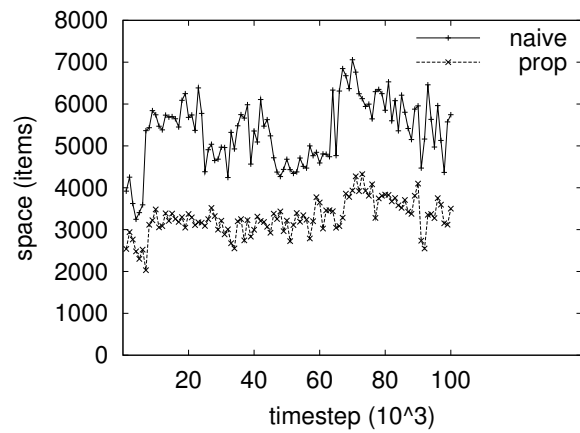
(b) data structure size
