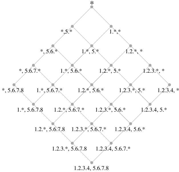
Figure 1: The lattice induced by the element (1.2.3.4, 5.6.7.8)
