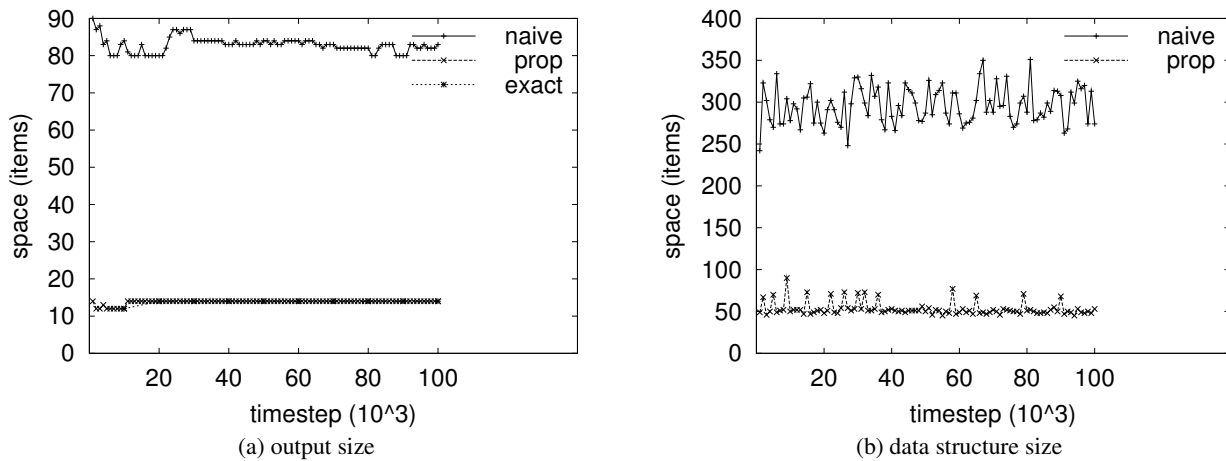
Figure 12: Comparison of output and data structure sizes from the online algorithms for the (smooth) split case, using FLOW with byte-level prefixes with ( \phi = 0.02, \epsilon = 0.01 ).
