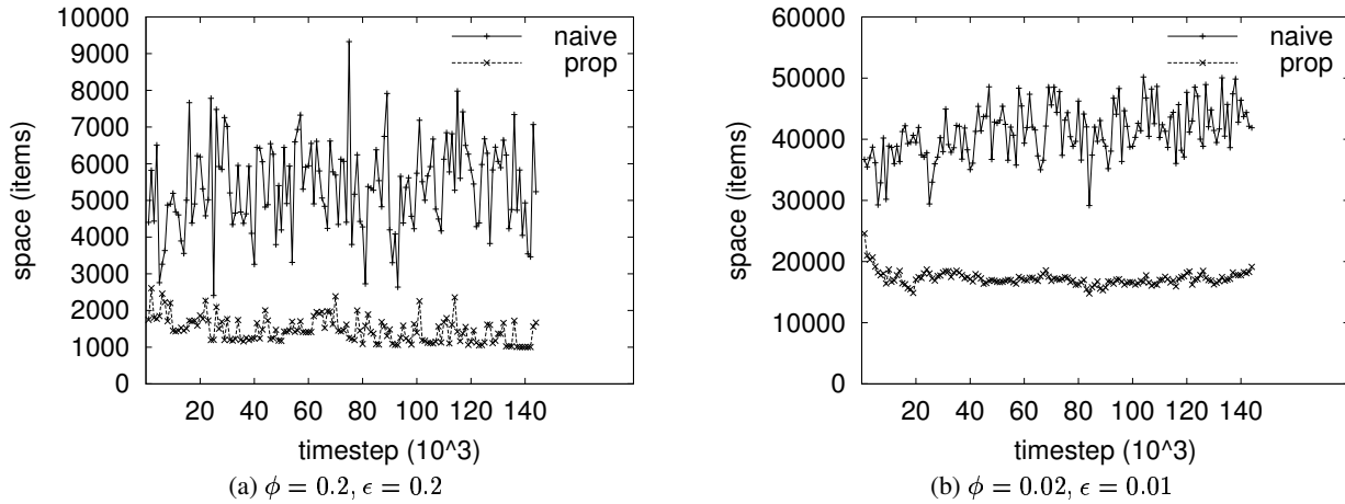
Figure 11: Comparison of data structure sizes from the online algorithms for the overlap case using PACKET with bit-level hierarchies.
