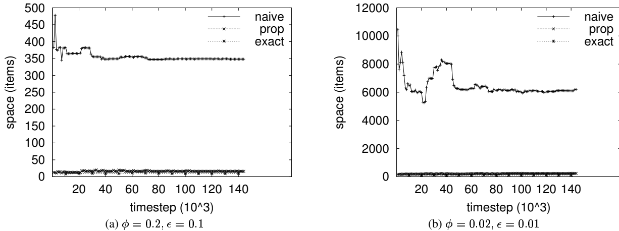
Figure 9: Comparison of output sizes from the online algorithms for the overlap case and the exact answer size using PACKET with bit-level hierarchies.
