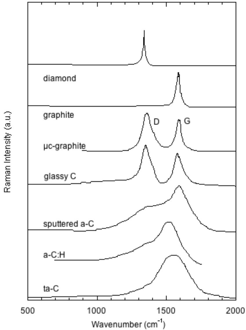
Figure 17: A typical Raman plot for different types of carbon. 26 Plots of this type can be used to determine \text{sp}^2/\text{sp}^3 fractions. The magnitude of peak shift can also be used to determine residual stress levels in the film
