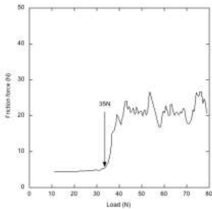
Figure 20c: DLC/TiN/Ti
