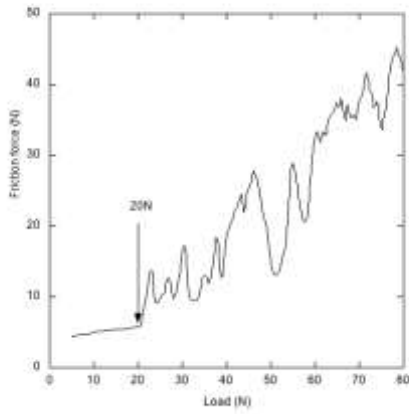
Figure 20a: DLC
