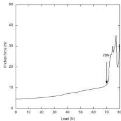
Figure 20d: DLC/Ti/TiN/TiCN
