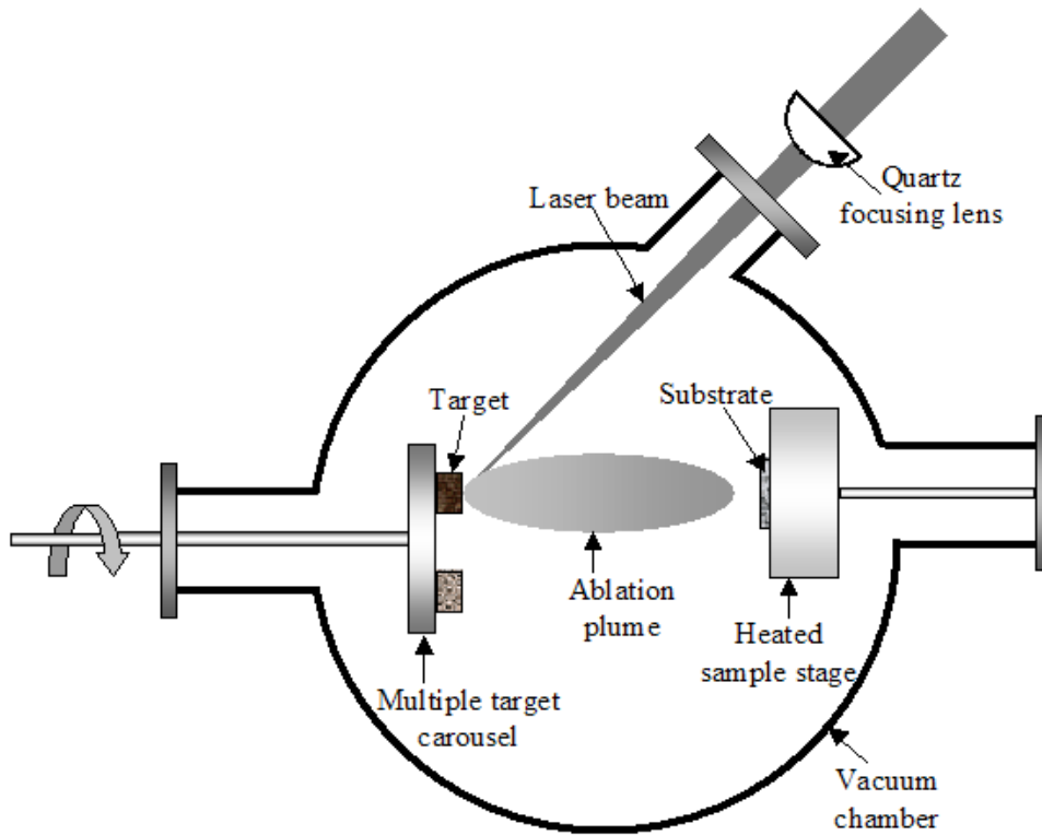
Figure 7: Schematic of a pulsed laser deposition system 44
