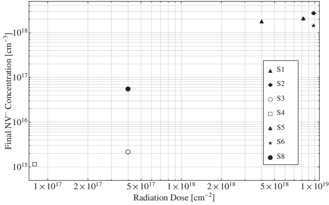
FIG. 5. NV^- concentrations near the surface as a function of dose for electron-irradiated samples after the final annealing at 1050 °C. The data are the same as used in Fig. 4(a).
