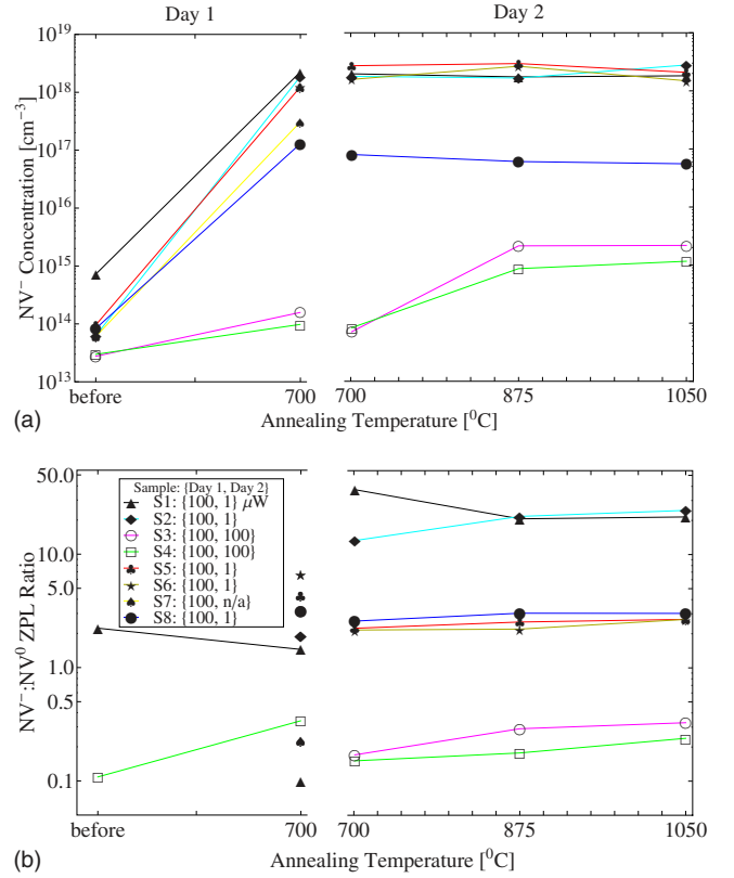
FIG. 4. (Color online) (a) \text{NV}^- concentrations of electron-irradiated samples as a function of annealing temperature. (b) \text{NV}^-:\text{NV}^0 ZPL intensity ratio of the same samples as a function of annealing temperature. The data were taken during two different runs on separate days. On each day the collection location for each sample was the same, but in between days the location changed. The laser power for the data on each day is indicated in the legend. Filled plot symbols are used for all samples with high-nitrogen content and empty symbols represent the two samples with \approx 1 ppm nitrogen. Error bars are not shown here but are discussed in the text.
