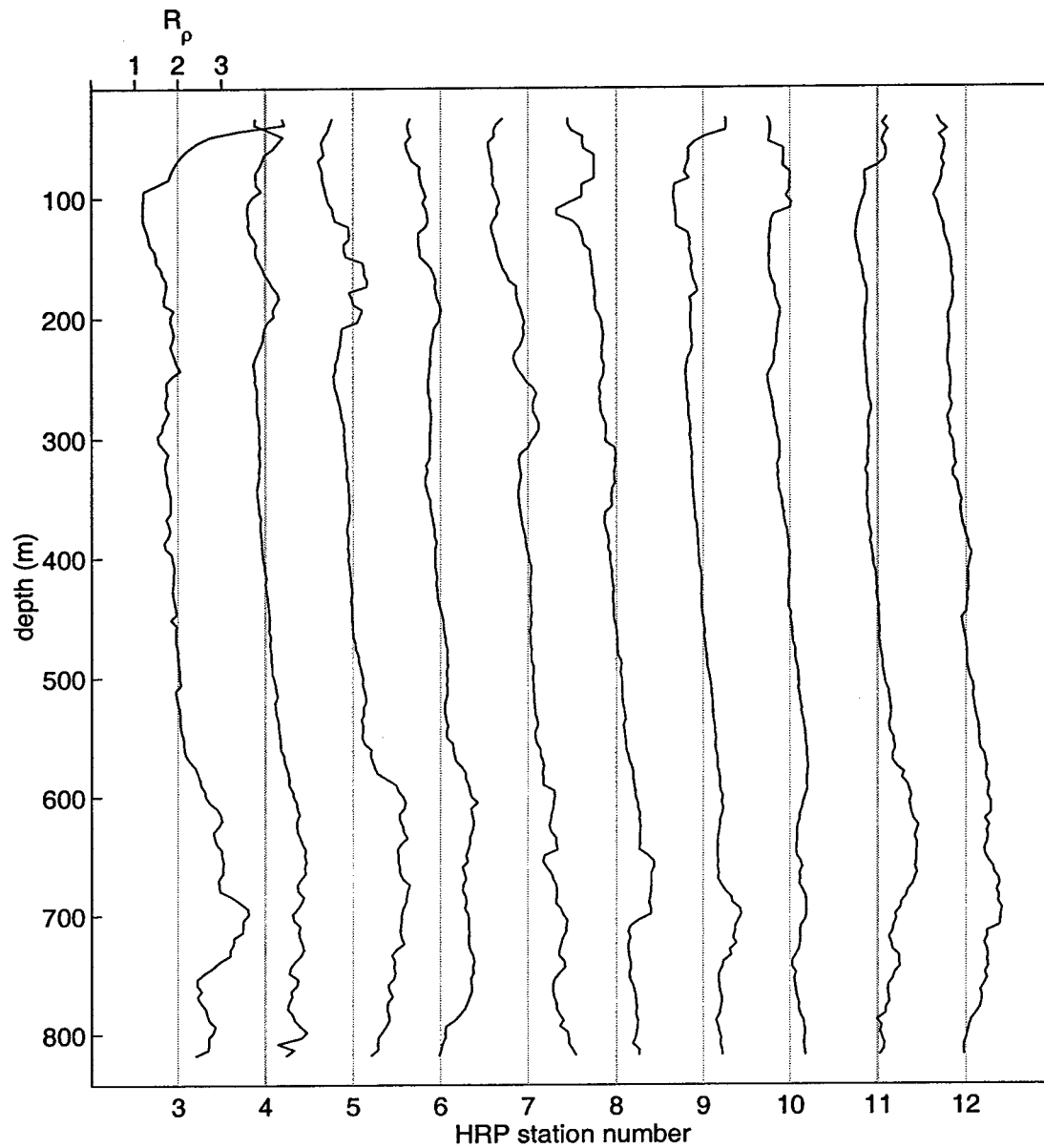
Figure 2.2: A section showing 10 profiles of the density ratio, R_\rho = \alpha \langle \Theta_z \rangle / (\beta \langle S_z \rangle)^{-1} . The gradients were calculated using a 5-m scale, smoothed using a 50-m running average. Stations 3-12 comprise the meridional section at the western edge of the survey. Each successive station is offset two R_\rho = 2 units and the reference value R_\rho = 2.0 is shown for each profile. There is large variability in the mixed layer and beneath z = 600 m due to intrusive features.
