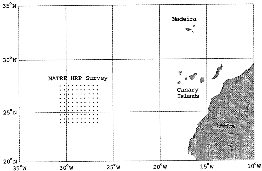
Figure 2.1: Location of the NATRE HRP survey. Over 150 dives were completed over 26 days. The survey consisted of the 100 station grid spanning the (400 \text{ km})^2 region shown. An additional 50 stations were tightly centered about (26^\circ\text{N}, -28^\circ\text{W}) . The HRP survey was completed two weeks prior to the tracer-release phase of the experiment.
