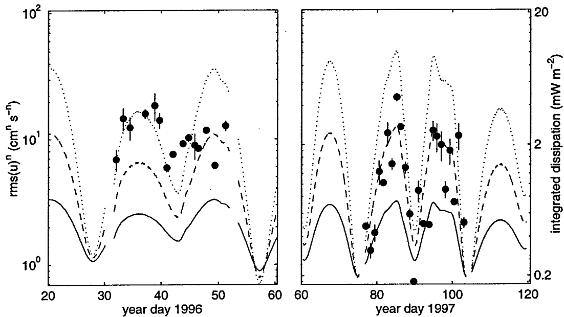
Figure 3.5: Comparison of column-integrated dissipation with power relations for the barotropic tidal speed. The rms tidal speed (solid line) is shown for general comparison purposes, but dynamical scalings suggest \epsilon \sim u^2 (dashed line) or \epsilon \sim u^3 (dotted line). The dissipation estimates \rho\epsilon were integrated to h_{ab} = 2000 m, and daily averages with standard errors are shown. The tidal velocity record was produced by the TPXO model of Egbert et al. (1994), and estimates were made along the survey tracks. Tidal estimates at a central location ( 18.5^\circ\text{W} , 21^\circ\text{S} ) were used for time intervals preceding and following survey periods.
