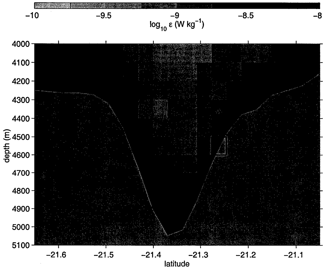
Figure 3.22: Section of dissipation across the canyon at 16^\circ\text{W} . Modeled \bar{\epsilon}(h_{ab}) profiles were used to generate the dissipation estimates along the floor, slopes, and upper flanks of the canyon. While the vertical derivative of \bar{\epsilon}(h_{ab}) favors downward advection in the canyon interior, upward w_* is favored in proximity to the sloping walls. A control volume taken along the slope will be characterized by a divergent vertical buoyancy-flux, as the turbulent heat-flux will exceed the flux through the seafloor.
