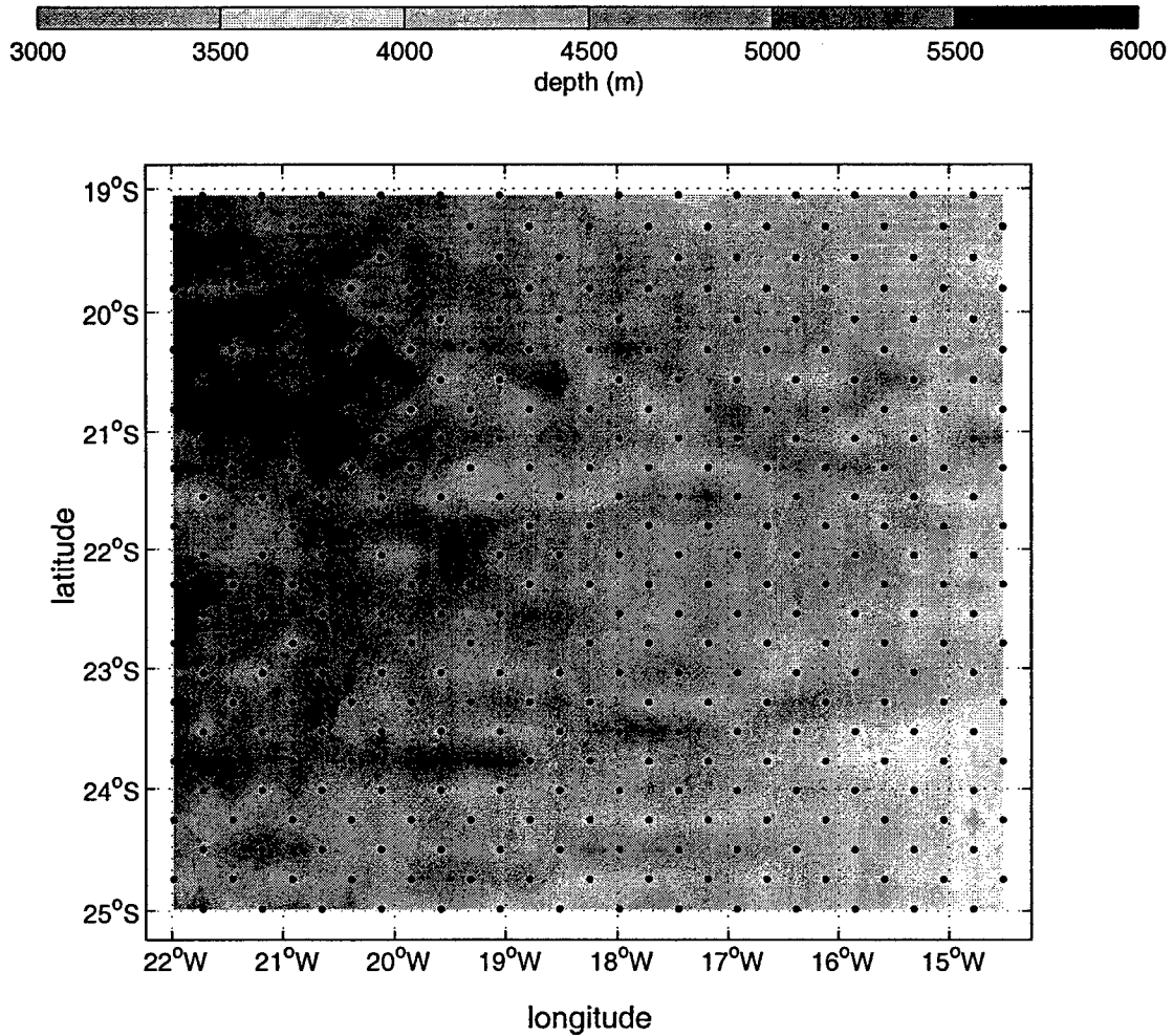
Figure 3.7: Map of the inversion domain. The staggered estimation grid is shown with the 0.25^\circ subsampled bathymetry. Hydrographic data were mapped onto this grid using polynomial fits. Modeled profiles of \bar{\epsilon}(h_{ab}) were assigned to each grid point according to bathymetric classification by first and second derivatives of the bottom topography.
