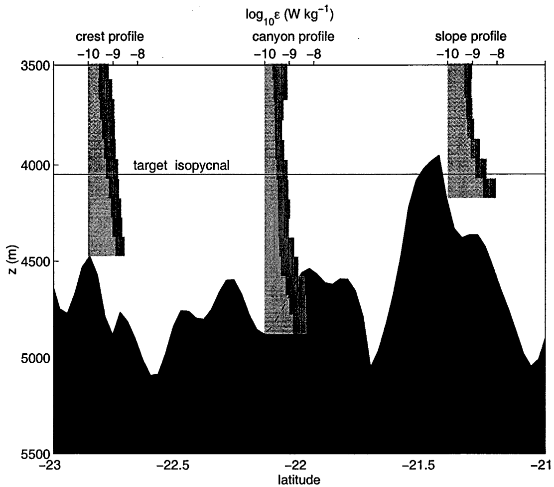
Figure 3.4: A section of meridional bathymetry at the longitude of the tracer injection ( 18.5^{\circ}\text{W} ). The target isopycnal ( \sigma_4 = 45.94 \text{ kg m}^{-3} ) of the tracer is also shown, as are the ensemble-averaged dissipation profiles for the 3 classes of bottom bathymetry. The target isopycnal experiences enhanced mixing rates along the slopes and peaks of FZ ridges. An estimate of mean dissipation for the target surface based on samples made above FZ canyons would be biased low.
