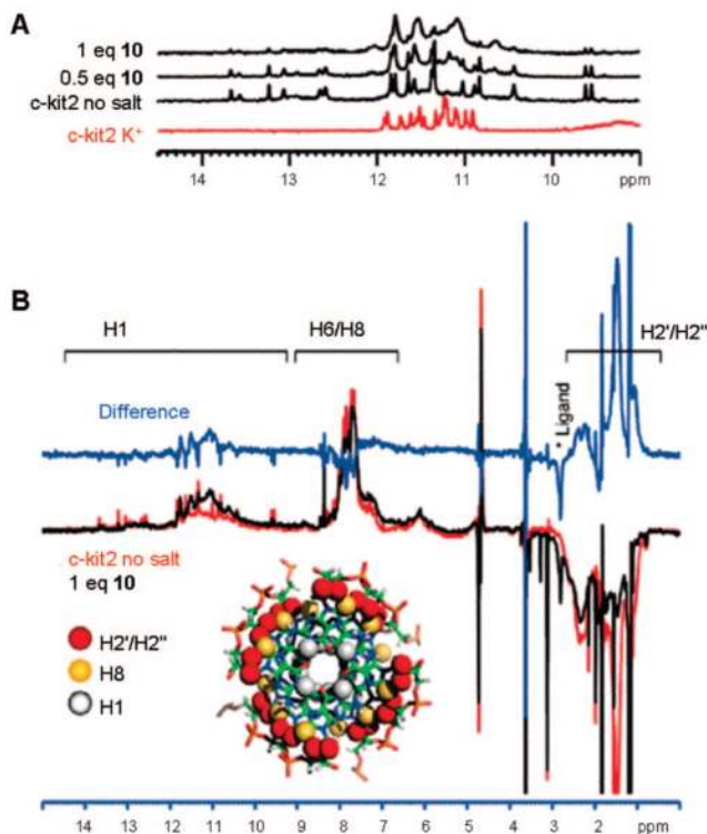
Figure 4. NMR titration study of a solution of 260 \mu M c-kit2 complexed with ligand 10 ; (A) the imino proton spectra of c-kit2 with 0, 0.5, 1 equiv of ligand 10 in the absence of added salt; bottom spectra (red) shows the imino proton spectrum of c-kit2 in presence K + . (B) 1D jump-and-return 1 H NMR spectra of c-kit2 in the absence (red) and in the presence (black) of 1 equiv of ligand 10 without added salt; the difference spectrum of the two is shown in blue with regions of different proton types indicated above; inset: a top view of a molecular model of three-layer G-tetrad in a parallel conformation 22 with H2'/H2'', H8 and H1 protons shown in red, gold and gray spheres.
