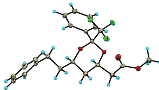
Fig. 1 X-ray structure of product 2a .
